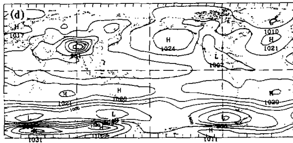
Fig. 3. Sea level air pressure (SLP) in (a), (b), coupled and (c), (d), uncoupled situation for January and July averaged for the last 20 years of the coupled integration. units: hPa.
