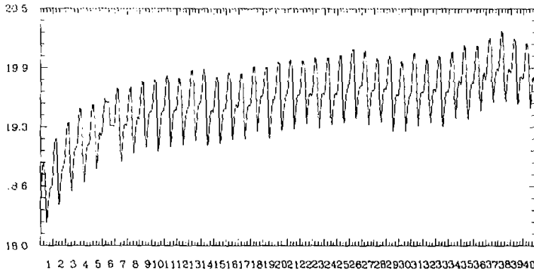
Fig. 1 The time evolution of monthly mean SST averaged over global ocean for the 40 years integration of the coupled model. unit: °C.
