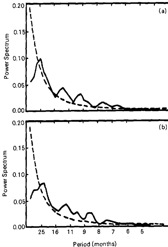
Fig. 1. The power spectra of monthly precipitation in the middle and lower reaches of the Yangtze River (a) and South China (b). The dashed line denotes 95% significance level.
