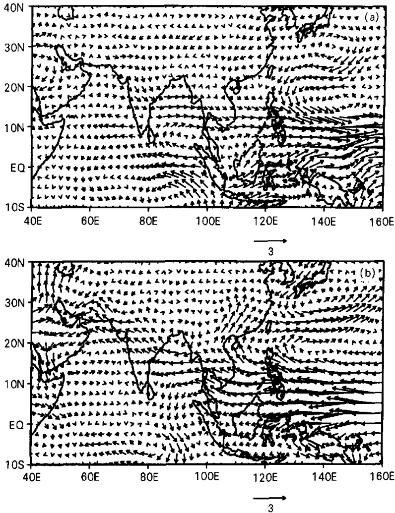
Fig. 7. Composite maps of the wind anomalies at 850 hPa in summer (JJA). (a) For strong East Asian winter monsoon cases (1962–1963, 1967–1968, 1975–1976, 1981–1982, 1985–1986, 1990–1991, 1996–1997), (b) for weak ones (1963–1964, 1972–1973, 1974–1975, 1982–1983, 1987–1988).
