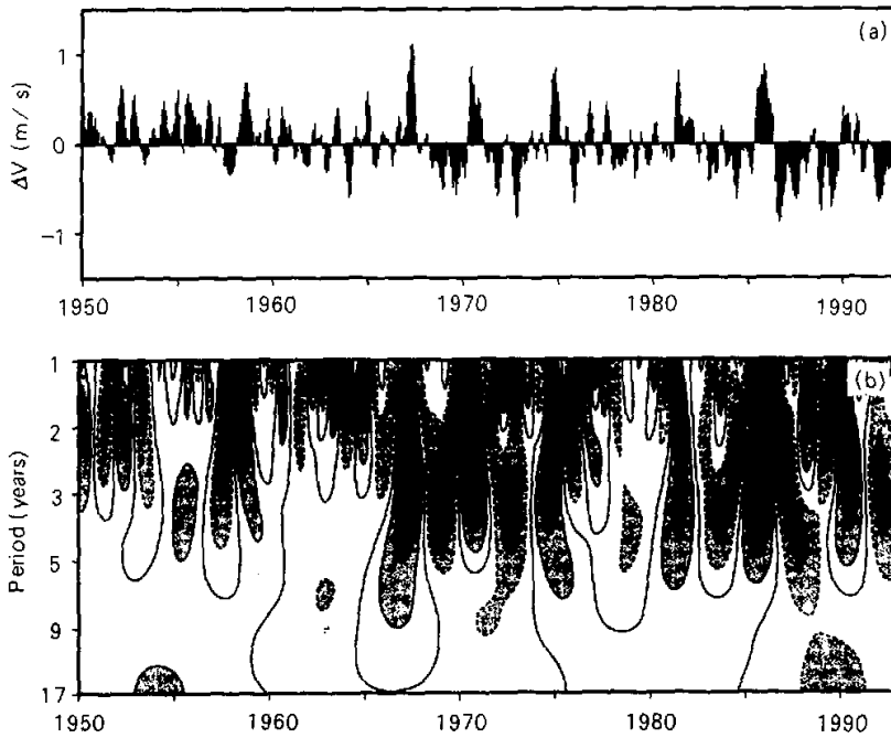
Fig. 3. Temporal variation of meridional wind anomalies in ( 20^{\circ} – 35^{\circ} N, 120^{\circ} – 150^{\circ} E) region (a) and its wavelet analysis results (b).
