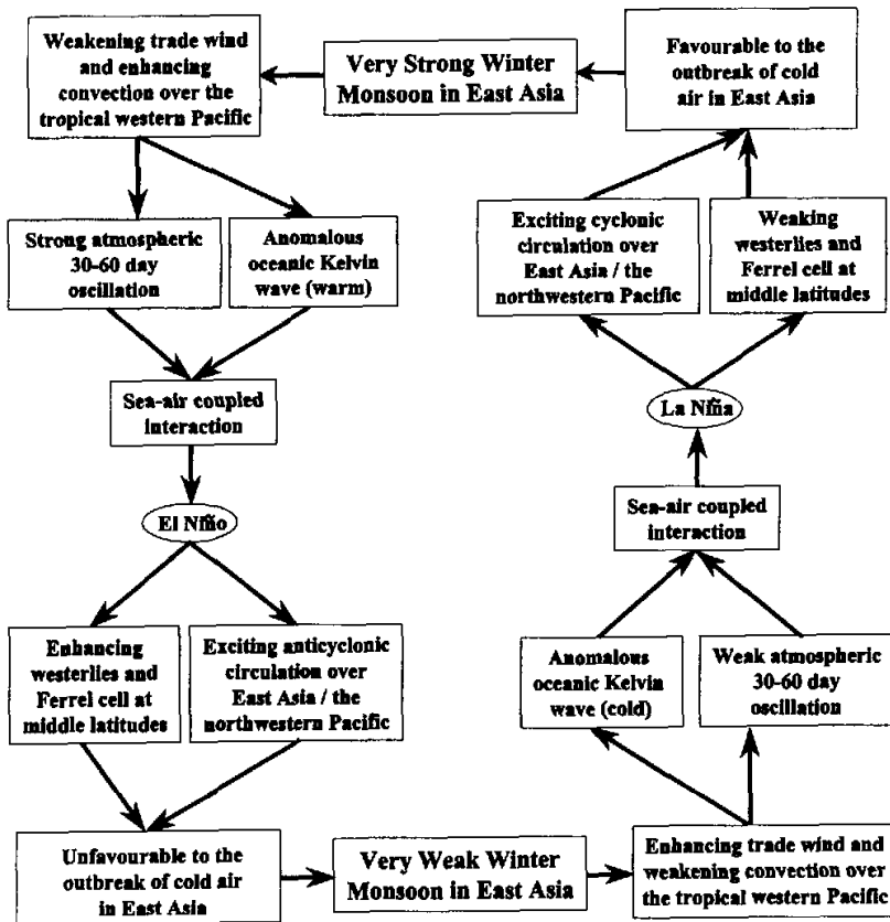
Fig. 6. Schematic diagram of the interactions between anomalous winter monsoon in East Asia and ENSO cycle.
