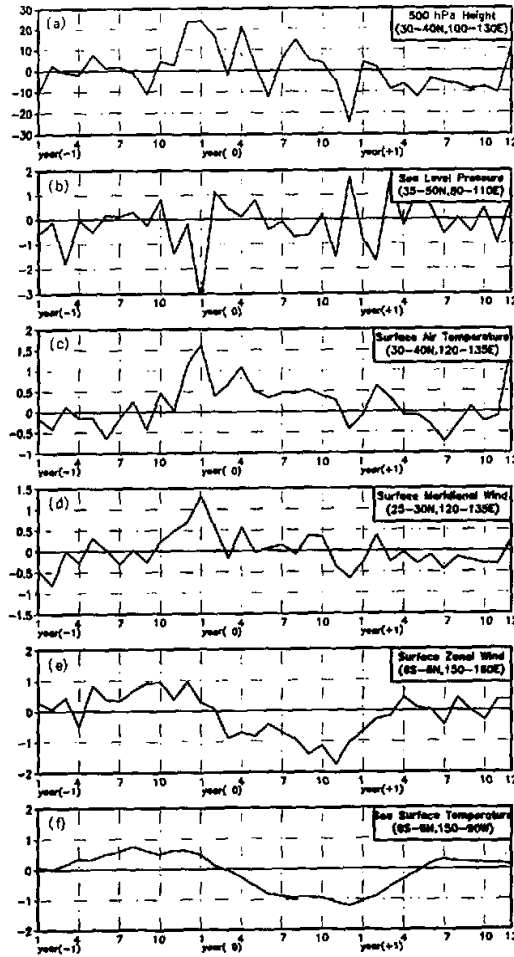
Fig. 5. Same as Fig. 1, but for composite La Niña case.
