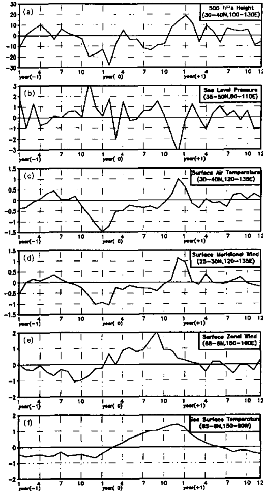
Fig. 4. The relationship between abnormal East-Asian winter monsoon and El Niño. The geopotential height anomalies at 500 hPa in the region (30°–40°N, 100°–130°E) (a), the surface pressure anomalies in the region (35°–50°N, 80°–110°E) (b), the surface air temperature anomalies in the region (30°–40°N, 120°–135°E) (c), the meridional wind anomalies in the region (25°–30°N, 120°–135°E), the zonal wind anomalies over the equatorial western Pacific region (6°S–6°N, 150°–160°E) (e) and the SSTA in the Niño 3 region (f) for composite El Niño case. The (–1), (0) and (+1) represent last year, present year and following year for the occurrence of El Niño, respectively.
