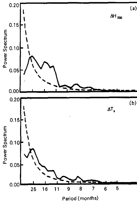
Fig. 2. The power spectra of the geopotential height variation at 500 hPa in the northwestern Pacific (20°–30°N, 120°–150°E) region (a) and surface temperature variation in the middle and lower reaches of the Yangtze River (b).
