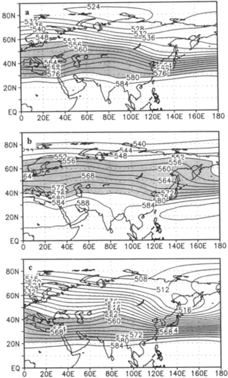
Fig. 4. The geographical distribution of the average 500 hPa geopotential height (in units of 10 m) for (a) April/ May, (b) June, and (c) January–February. Areas with values larger than 552 and smaller than 580 are shaded.
