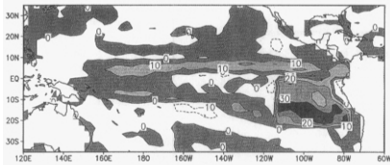
Fig. 5. Differences of the simulated annual mean low-level cloud covers between CldSen1 and FGCM-Exp. Contour interval is 10%, and positive values are shaded.
