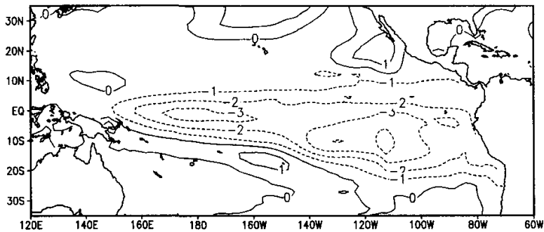
Fig. 6. Differences of the simulated annual mean SSTs between CldSen1 and FGCM-Exp. Contour interval is 1°C. Negative values are expressed by dashed lines.
