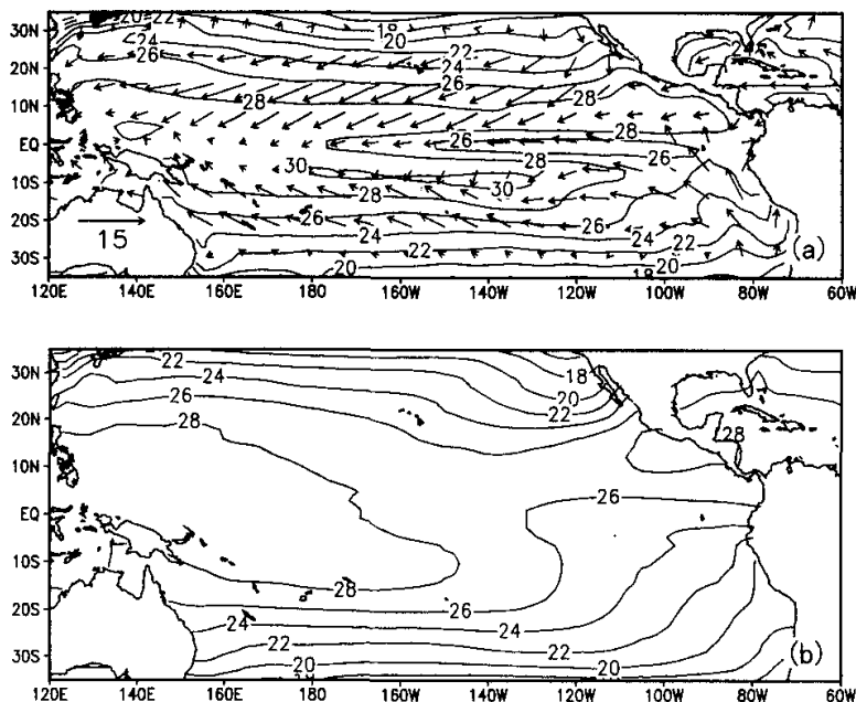
Fig. 1. (a) The simulated annual mean SST and surface wind in FGCM-Exp, (b) the observed annual mean SST. The contour interval of isotherms is 2°C. The simulated surface wind is expressed by vectors with the vector scale shown at the bottom-left corner in (a).
