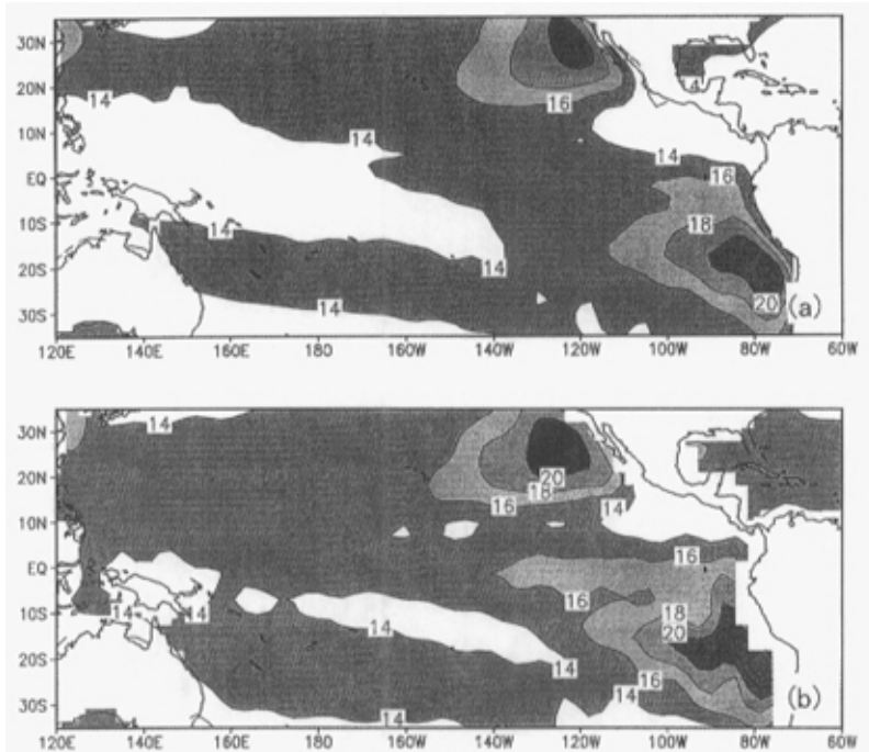
Fig. 3. The observed (a) and simulated (b) annual mean bulk stability of the low troposphere. The contour interval is 2°C. The values greater than 14°C are shaded.
