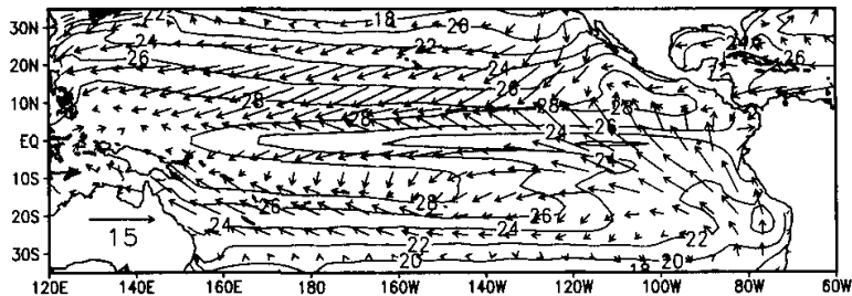
Fig. 7. The annual mean SSTs and surface wind simulated by CldSen1. The SST is expressed by isotherms with contour interval 2°C. The surface wind is expressed by vectors with the vector scale at the bottom-left corner.
