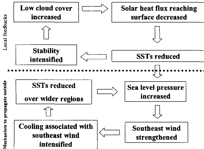
Fig. 11. The sketch map of the mechanisms involving impacts of low-level cloud covers over the region off Peru.
