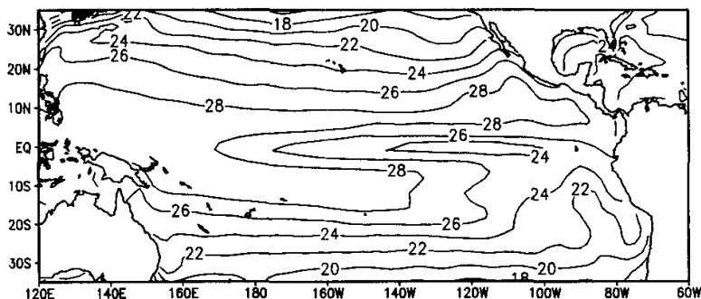
Fig. 10. The annual mean SSTs simulated by SstSen. Contour interval is 2^{\circ}\text{C} .
