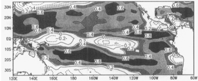
Fig. 4. The distribution of correlation coefficients between the low-level cloud cover and the bulk stability of the low troposphere based on the ISCCP data and the NCEP reanalysis from 1984 through 1993. The bulk stability is defined as the difference of potential temperature between 700 hPa and 1000 hPa. Areas where coefficients reach the 99% confidence level test are shaded. The contour interval is 0.2.
