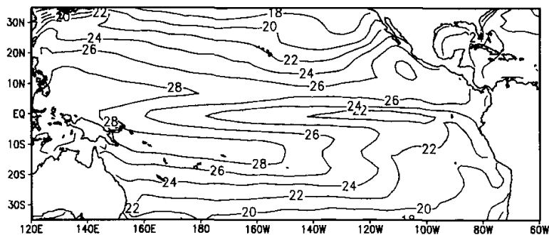
Fig. 9. The annual mean SST simulated by CldSen2. Contour interval is 2^{\circ}\text{C} .
