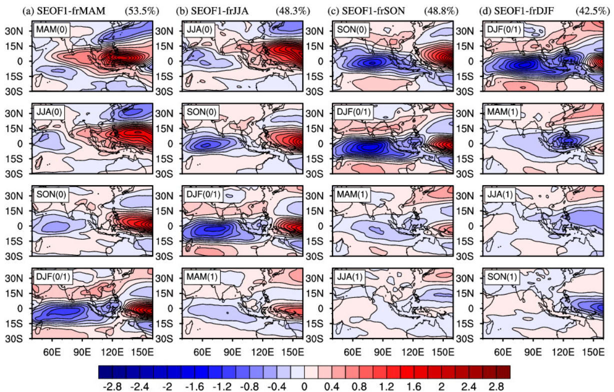
Fig. S1. The first SEOF spatial patterns of AAM U850 anomalies (units: \text{m s}^{-1} ) as derived from different initial seasons in BCC_CSM1.1M data: (a) SEOF1-frMAM; (b) SEOF1-frJJA; (c) SEOF1-frSON; (d) SEOF1-frDJF.
