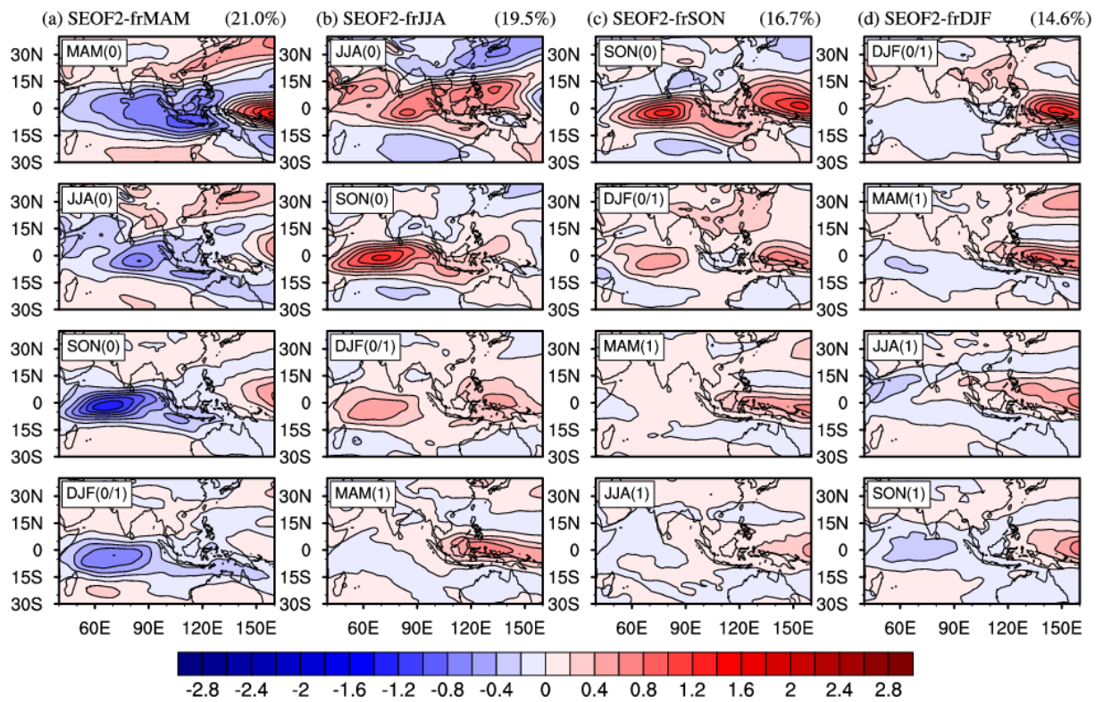
Fig. S2. Same as Fig. S1, but for the second SEOF.
