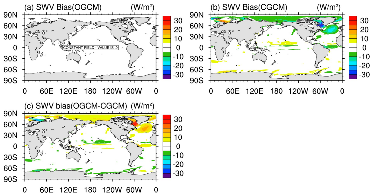
Fig. S1. The pattern of shortwave flux bias relative to control experiment (a) OGCM, (b) CGCM, and (c) their difference (units: \text{W m}^{-2} ).
