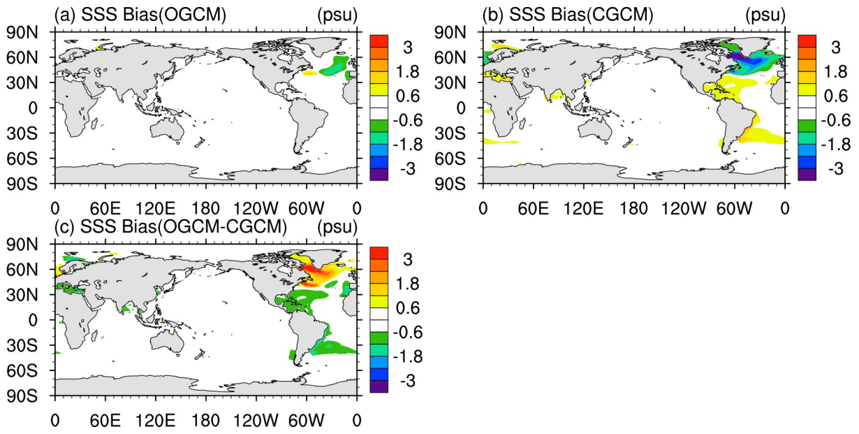
Fig. S2. The pattern of sea surface salinity bias relative to control experiment (a) OGCM, (b) CGCM, and (c) their difference (units: psu).
