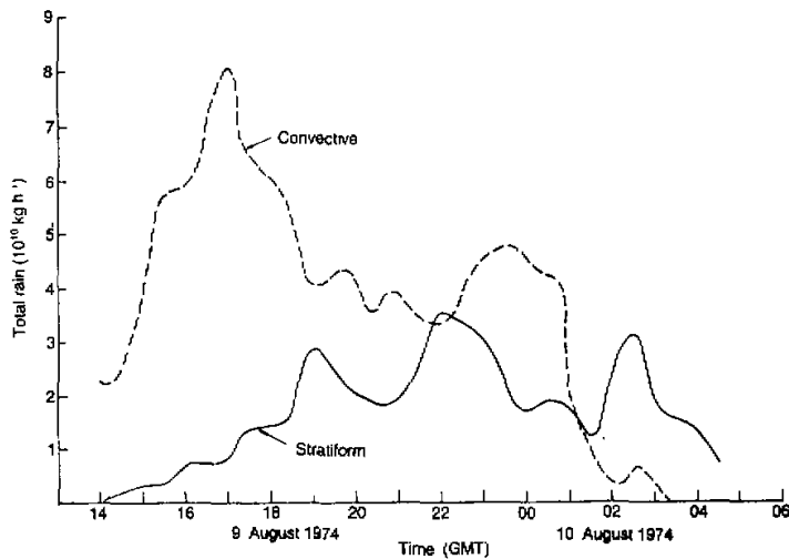
Fig. 4. Time variation of total rain integrated over areas covered by the convective and stratiform regions of the 9–10 August 1974 GATE squall system.
