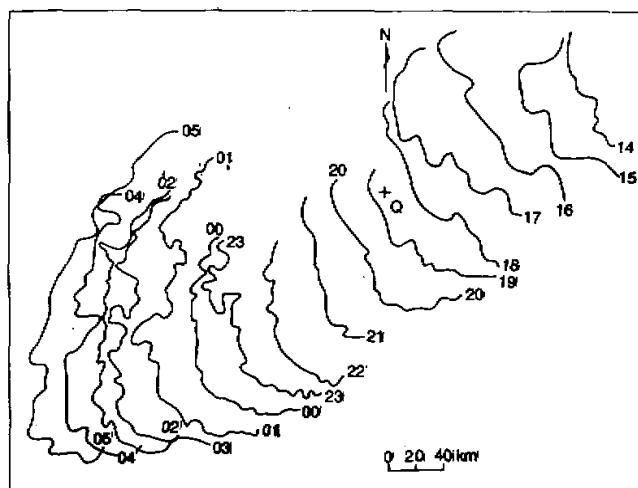
Fig. 1. Isochrones of leading edge of convective radar-echo zone of the GATE squall line. Times are to the nearest hour (GMT). Data from 1408–1800 GMT are from radar aboard the ship Quadra (Q). Data from 1900–0500 GMT are from the Oceanographer (O).
