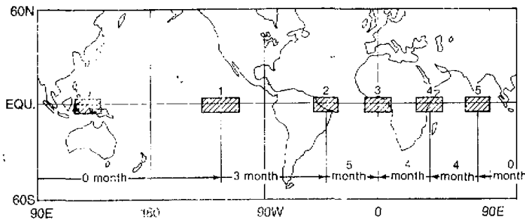
Fig. 1. Six areas in the global tropics studied in this paper. 1: eastern Pacific; 2: western Atlantic; 3: eastern Atlantic; 4: western Indian Ocean; 5: central Indian Ocean; 6: western Pacific.
