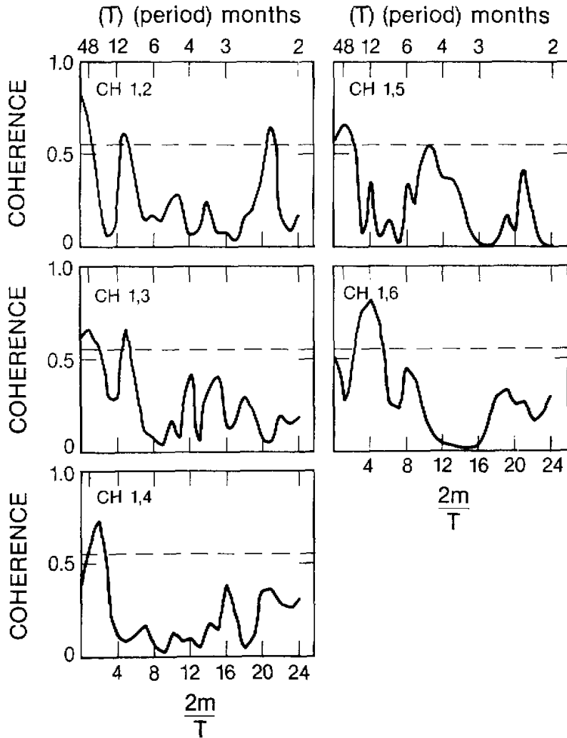
Fig. 6. Coherence spectra between area I and others as a function of period and frequency. The dashed line indicates the 95% confidence level.
