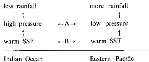
Fig. 5. Schematic diagram of correlations between rainfall, surface pressure and surface temperature in the areas of the eastern Pacific and Indian Ocean.
