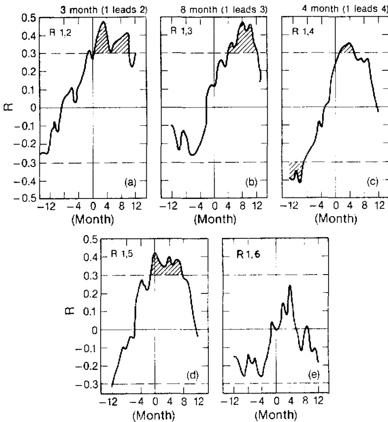
Fig. 4. Cross-correlation coefficients between area 1 and other areas as the function of time lag ( -12 to +12 months). Positive numbers mean that area 1 leads. Shaded areas indicate the range reaching 95% confidence.
