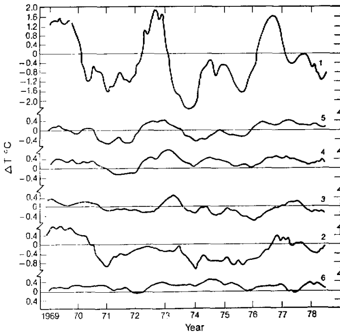
Fig. 3. Low-pass filtered curves of monthly sea surface temperature anomalies in six areas.
