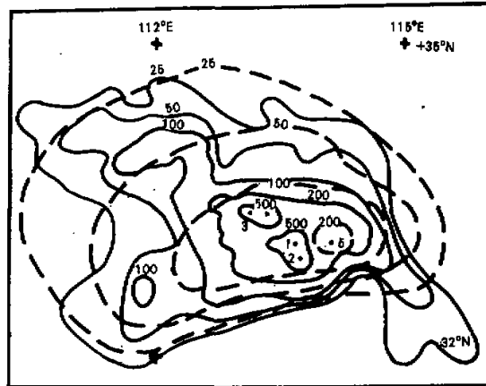
Fig.1. The 24-h observed rainfall (mm) ending at 0000 GMT 8, August 1975. Dashed lines are isopluvials based only on data of synoptic stations and solid ones with data of climatological and hydrological stations in addition. The five spots are: 1–Linzhuang, 2–Laojun, 3–Guolin, 4–Yanglou, 5–Zhumadian, respectively.
