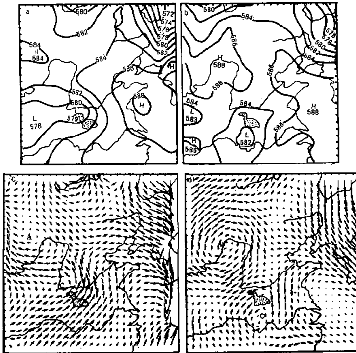
Fig.4. As in Fig.3, but for 500 hPa.
