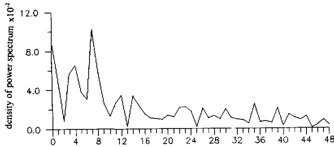
Fig. 3. The spectrum of anomalous TAV averaged for the whole basin for the period 1959–1988 with a maximum lag by 48 bimonths
