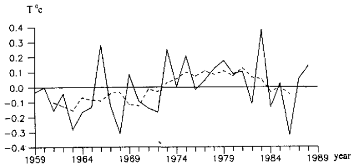
Fig. 4. Time sequence of yearly mean of anomalous TAV (solid line) from 1959 to 1988 and the 5-year running means (dashed lines) of it.
