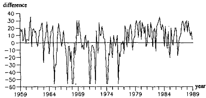
Fig. 6. Time sequence of difference between the westernmost longitude of the western Pacific subtropical high ridge and longitude 125°E from 1959 to 1988.
