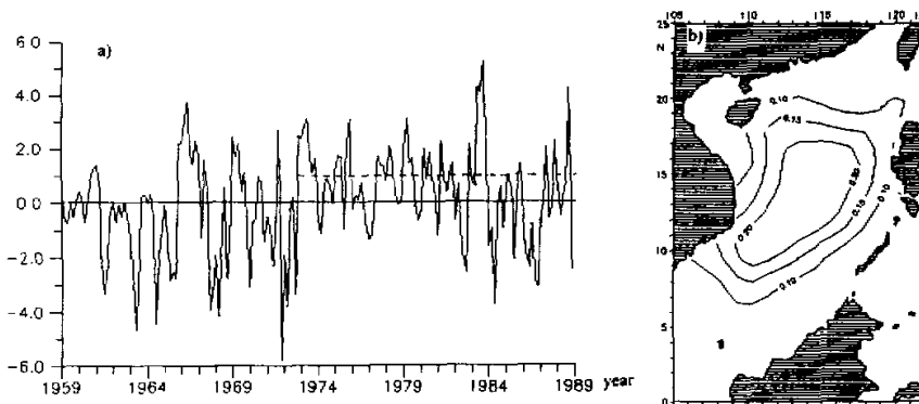
Fig. 2. First empirical orthogonal function of anomalous TAV with time function (a) and spatial patterns (b) displayed.
