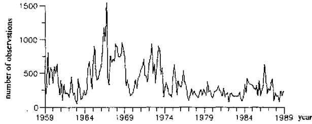
Fig. 1. Time sequence of bimonthly number of temperature/depth observations in the South China Sea from 1959 to 1988.
