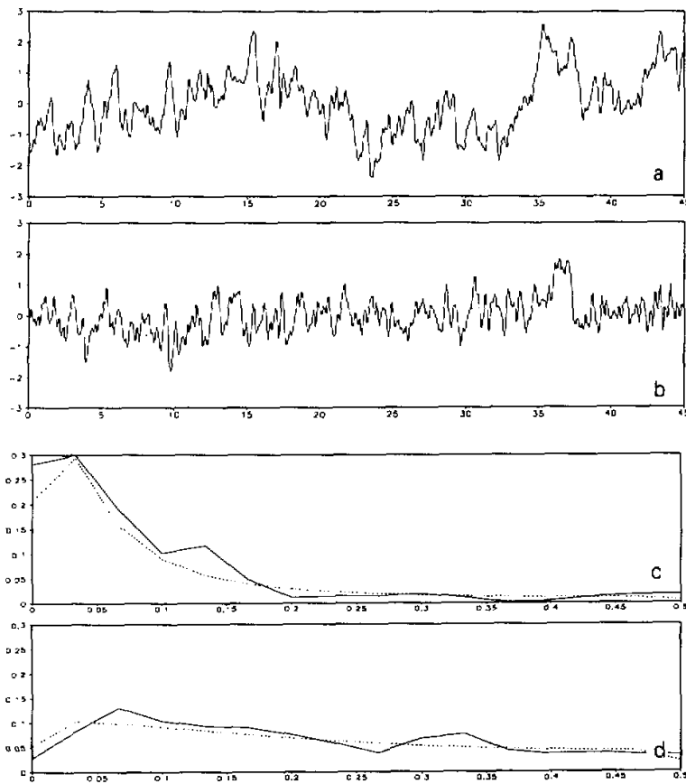
Fig. 5. Time evolution of SST anomaly averaged over the region of 157.5\text{--}172.5^\circ\text{E} , 4^\circ\text{N}\text{--}4^\circ\text{S} for the 45 years for (a) prescribed and (b) diagnostic cloud run. Unit: K. The power spectra for (a) and (b) are shown in (c) and (d) respectively. The vertical coordinate in (c) and (d) is the spectral power density and the dashed line is the corresponding spectrum of red noise.
