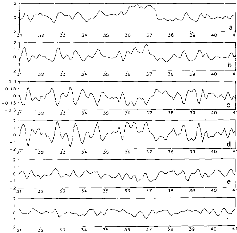
Fig. 7. Same as Fig. 6 except for the diagnostic cloud run.
