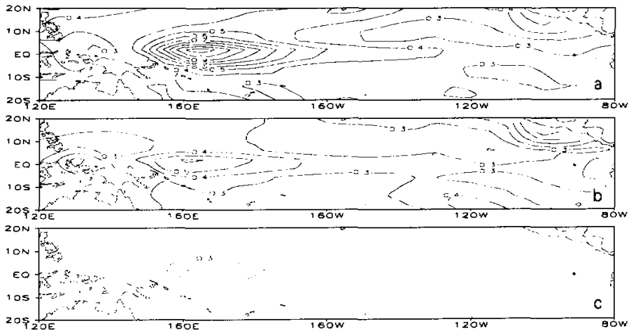
Fig. 1. Geographic distributions of the standard deviation of monthly mean SST from (a) prescribed cloud, (b) diagnosed cloud integration and (c) the difference between the prescribed and diagnosed cloud run. Unit: K.
