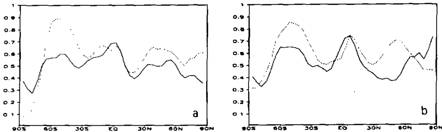
Fig. 2. Zonal-mean total cloud cover fraction of the AMIP run and ISCCP data for (a) January and (b) July. The dashed line is for ISCCP data.
