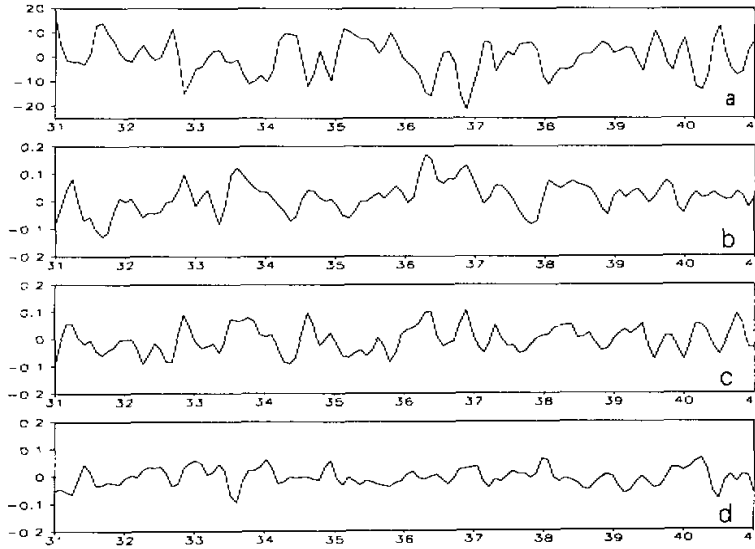
Fig. 8. Time evolution of the regionally averaged anomaly of (a) net SW flux, (b) high, (c) middle, and (d) low cloud cover for the diagnostic cloud run. Unit: SW: W / m^2 , positive for downward.
