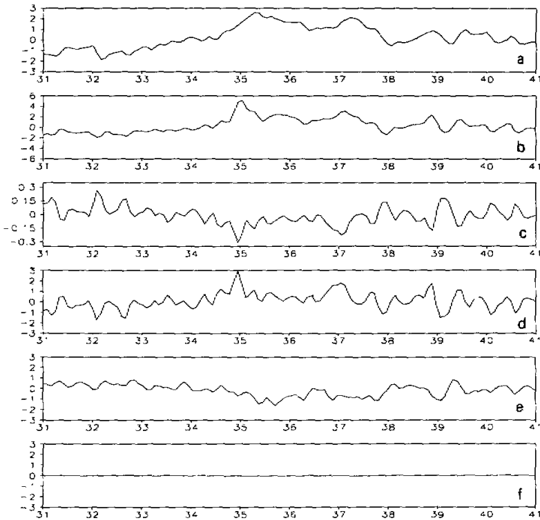
Fig. 6. Time evolution of anomaly of (a) SST, (b) zonal wind and (c) vertical velocity at the interface between the top layer and second layer in ocean, the tendencies of SST due to (d) upwelling / downwelling, (e) latent heat flux and (f) net SW flux for the prescribed cloud run over the region of 157.5^{\circ}\text{E} — 172.5^{\circ}\text{E} , 4^{\circ}\text{N} — 4^{\circ}\text{S} . Units: wind: \text{m/s} ; vertical velocity: \text{m/day} , positive for upward; all tendencies: 0.01 \text{ K/day} ; latent heat flux: positive for upward.
