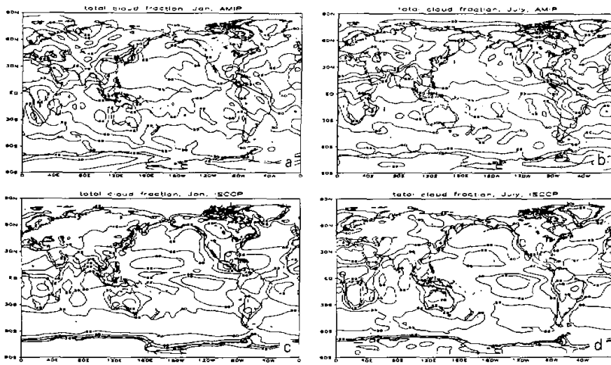
Fig. 3. The global distribution of total cloud cover fraction of the AMIP run for (a) January and (b) July, averaged for the ten years. (c) January and (d) July climatology of ISCCP. Unit: percentage (%), contour interval: 20.
