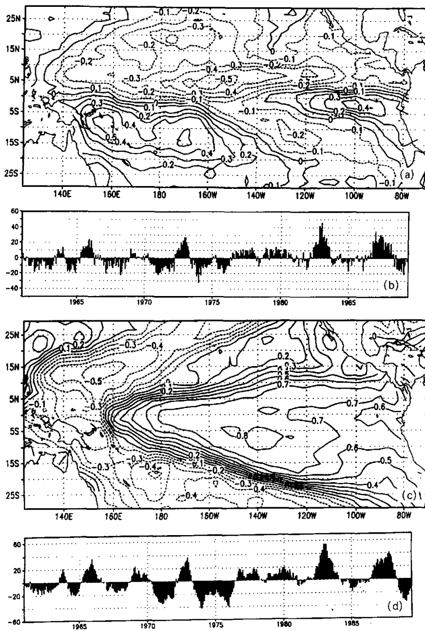
Fig. 5. Same as Fig. 3 but for the meridional wind stress anomalies prior to SSTA by one month.
