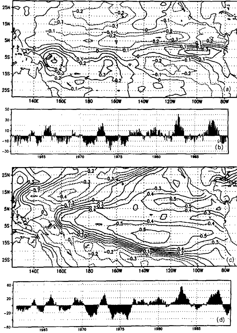
Fig. 3. Coupling patterns of SSTA (c) and the meridional wind stress anomalies prior to SSTA by six months (a) for the first mode with the largest singular value, and evolutions of the time coefficients of coupling patterns of SSTA (d) and meridional wind stress anomalies (b).
