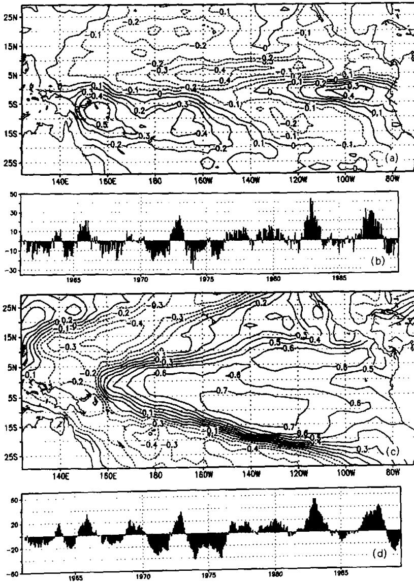
Fig. 4. Same as Fig. 3 but for the meridional wind stress anomalies prior to SSTA by three months.
