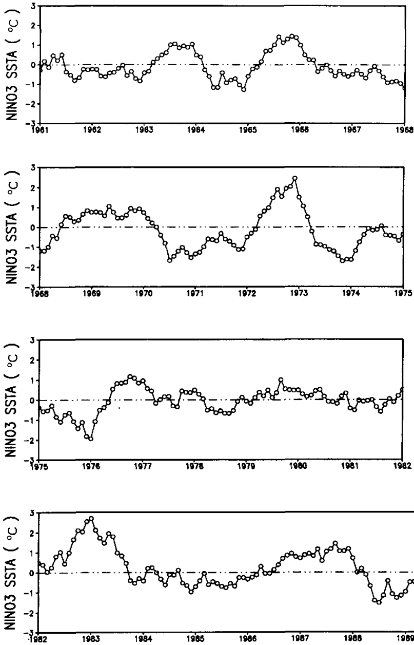
Fig. 1. The time evolution of the monthly NINO3 SSTA (1961–1989).
