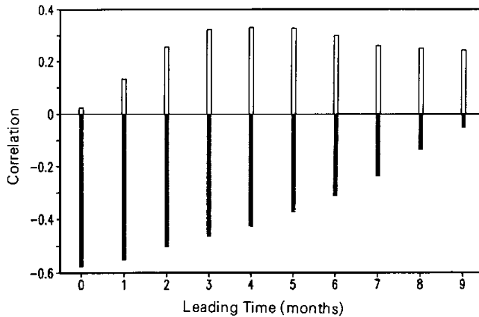
Fig. 6. Correlation coefficients of NINO3 SSTA with leading zonal wind stress anomalies averaged over the area 124^{\circ}\text{--}160^{\circ}\text{E} , 10^{\circ}\text{S--}10^{\circ}\text{N} (outline bar) and with the difference between leading meridional wind stress anomalies averaged over the area 120^{\circ}\text{--}86^{\circ}\text{W} , 3^{\circ}\text{--}9^{\circ}\text{N} and those averaged over the area 120^{\circ}\text{--}86^{\circ}\text{W} , 5^{\circ}\text{S--}1^{\circ}\text{N} (filled bar).
