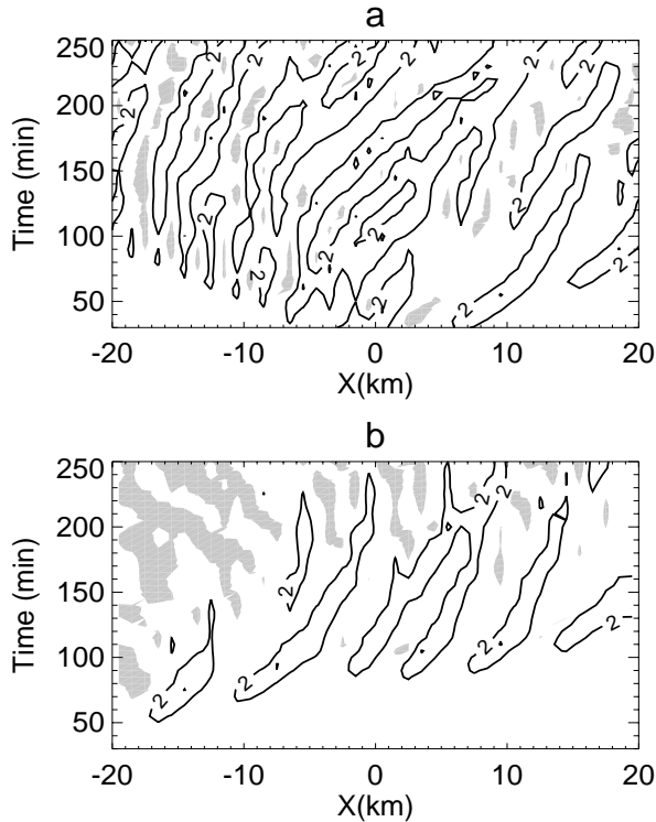
Fig. 6. The Hovmöller diagrams of \bar{u}_z obtained from (a) the large domain simulation with periodic boundary conditions and (b) from the simulation with the LBC configuration CR. The negative contours are shaded.
