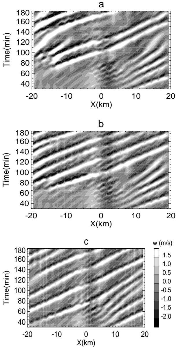
Fig. 8. The Hovmöller diagrams of vertical velocities from three hilly terrain simulations with (a) CR configuration, (b) SR, and (c) PP. The large scale geostrophic wind is 10 \text{ m s}^{-1} and the model surface is constantly heated. The sections are all taken at the 600-m model level.
