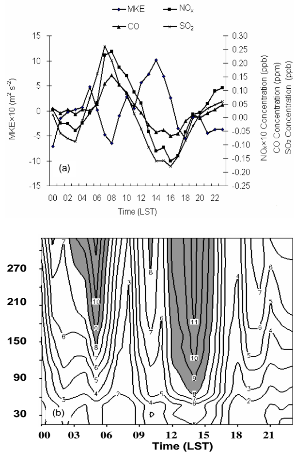
Fig. 4. Diurnal evolution of E_{MK} at the IAP site for January–March 2001 in Beijing. (a) Standardized variables of the mean kinetic energy and pollutant concentrations averaged over 8–320 m; (b) Vertical distribution (8–320 m) of the diurnal variation of mean kinetic energy.
