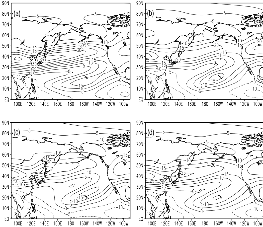
Fig. 1. 1979–2022 mean 200-hPa zonal wind ( \text{m s}^{-1} ) in (a) June, (b) July, (c) August, and (d) JJA.
