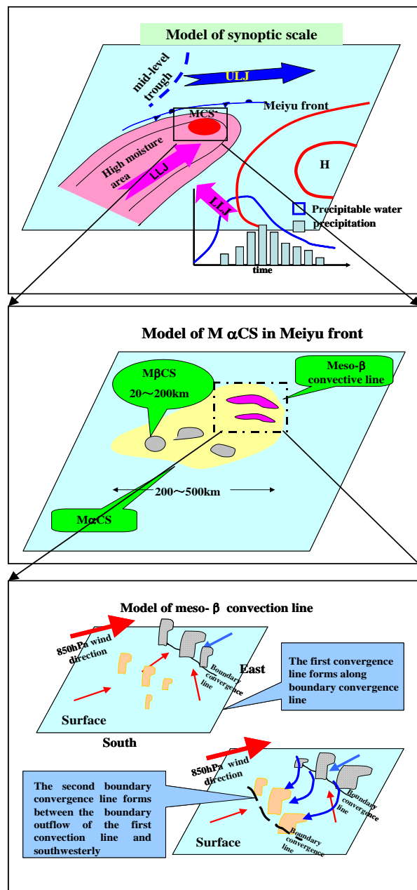
Fig. 10. Multi-scale conceptual model of heavy rainfall in the mei-yu front: (a) Synoptic model, (b) Meso- \alpha model, and (c) Meso- \beta convection line model.
