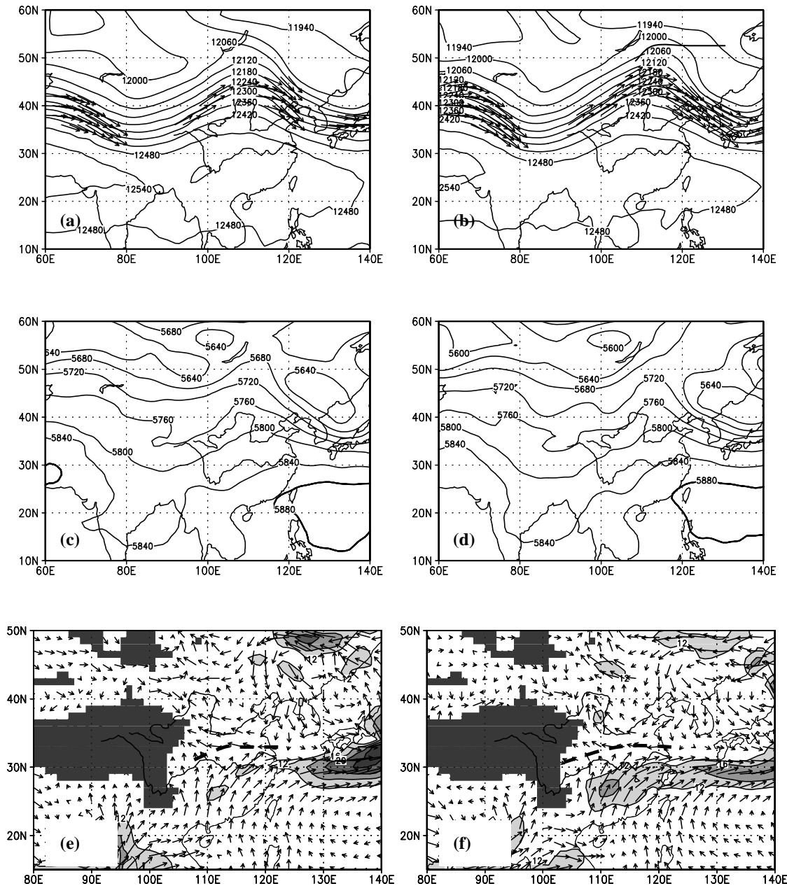
Fig. 2. Geopotential height in gpm and wind greater than 40 \text{ m s}^{-1} at 200 hPa (upper panel), Geopotential height in gpm at 500 hPa (middle panel), and wind field at 850 hPa with wind greater than 12 \text{ m s}^{-1} being shaded (lower panel, the deep shaded area is topography greater than 1500 m, bold dashed line is the shear line). (a), (c), (e) are at 2000 LST 20 June and (b), (d), (f) are at 0800 LST 21 June 2002.
