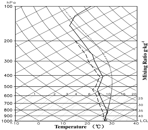
Fig. 9. Composite sounding on skew T -log p diagrams, temperature (solid line), dew point (dashed line), and path in (T, p) space taken by surface parcel as it ascends (dotted line). The pressure is plotted in hPa on the ordinate and temperature is plotted on a skewed abscissa in ^{\circ}\text{C} at Anqing station for 0800 LST 21 June 2002.
