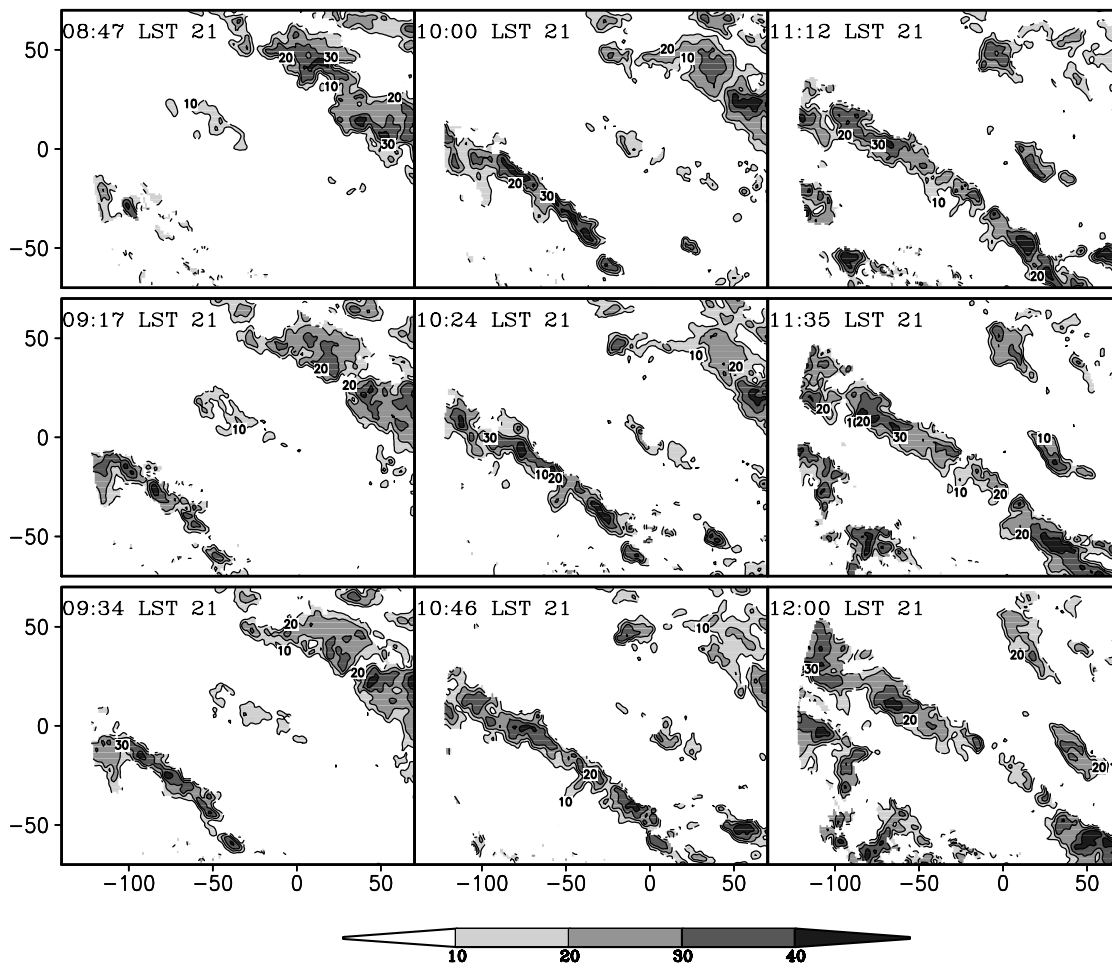
Fig. 8. As in Fig. 6 for 0800–1200 LST 21 June 2002.
