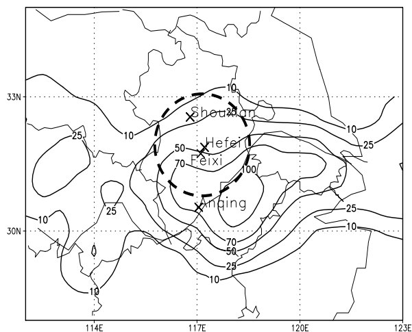
Fig. 1. The observed 36-h precipitation of 0800 LST 20 June–2000 LST 21 June 2002. The cross marks indicate the location of Shouxian, Hefei, Feixi and Anqing stations. The dashed circle shows the observation area by the Hefei radar. (units: mm)
