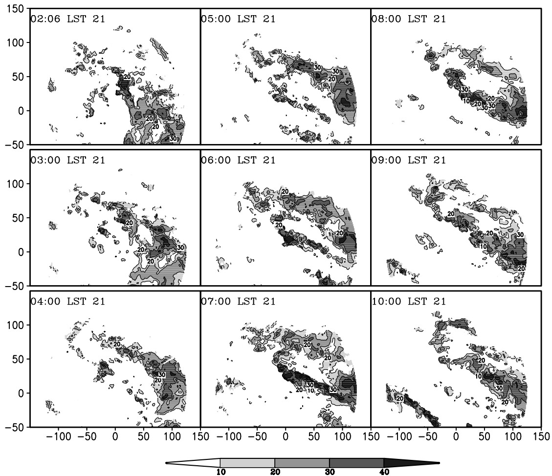
Fig. 6. The reflectivity in dBZ at 2 km ASL by the Hefei radar during 0200–1000 LST 21 June 2002. The origin (0,0) represents the location of the Hefei radar.
