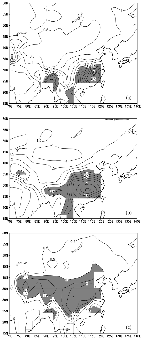
Fig. 8. Same as Fig. 6, but for spring.
