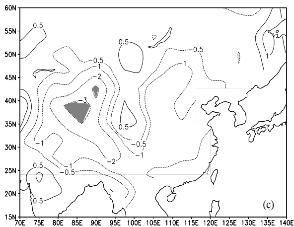
Fig. 4. Same as Fig. 1, but for summer.
