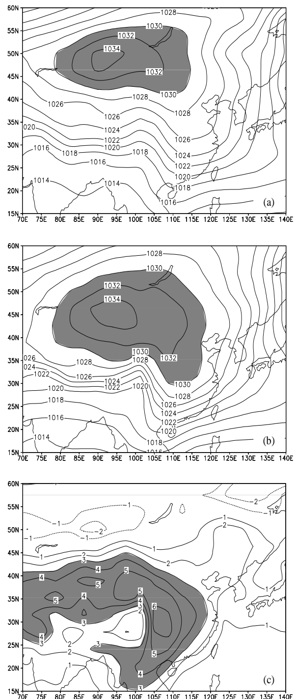
Fig. 12. Same as Fig. 11, but for winter.
