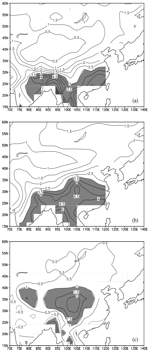
Fig. 6. Annual terrestrial precipitation climatology throughout 1961 to 1990 (units: \text{mm d}^{-1} ). (a) CRU data, (b) the seven-model ensemble mean, and (c) the nine-point running average differences of the ensemble mean against the CRU data. The regional minimum and/or maximum centers, with variational value level, are shaded.
