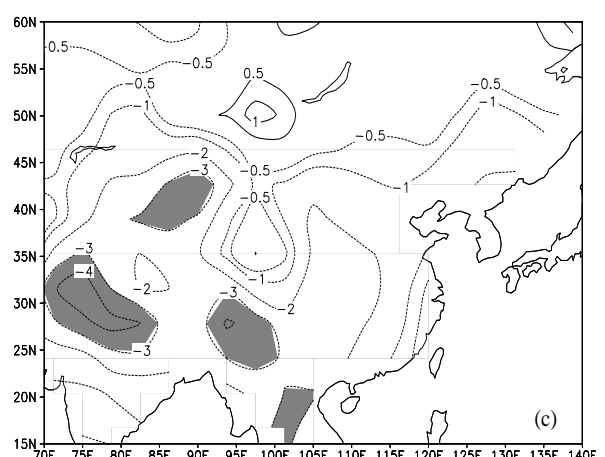
Fig. 5. Same as Fig. 1, but for autumn.
