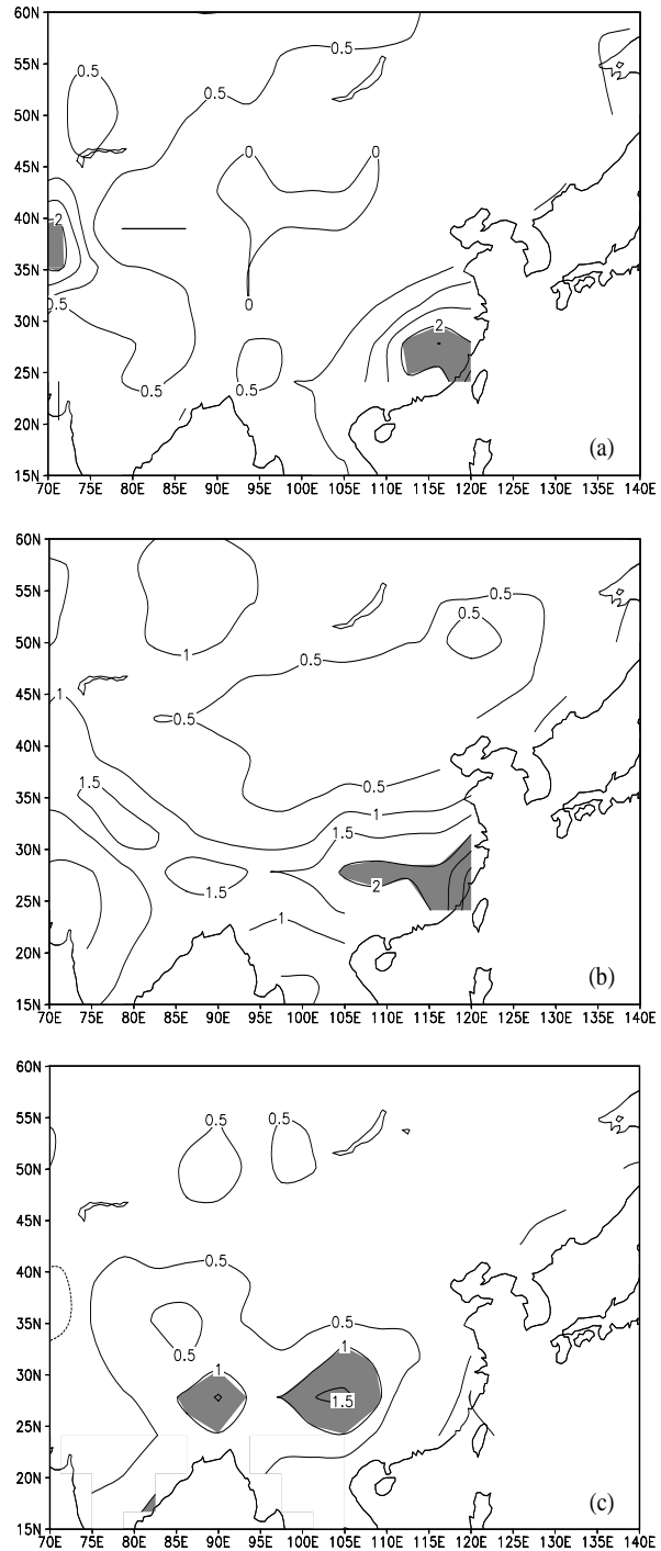
Fig. 7. Same as Fig. 6, but for winter.
