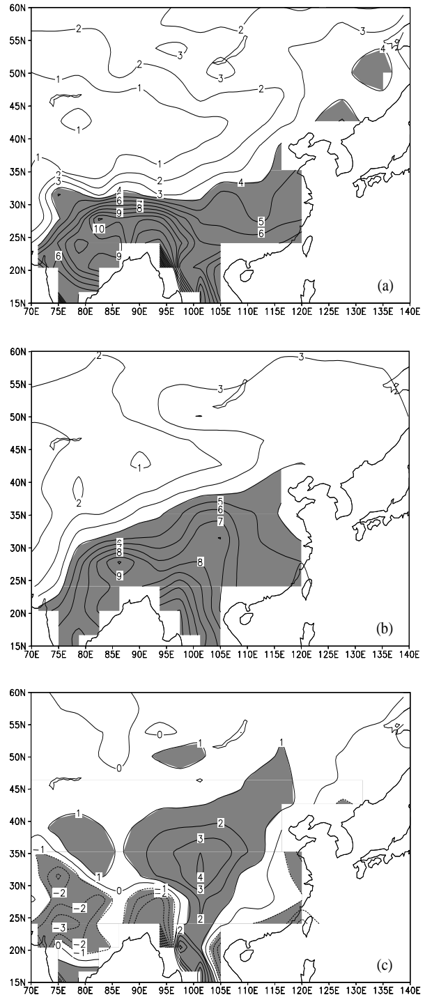
Fig. 9. Same as Fig. 6, but for summer.
