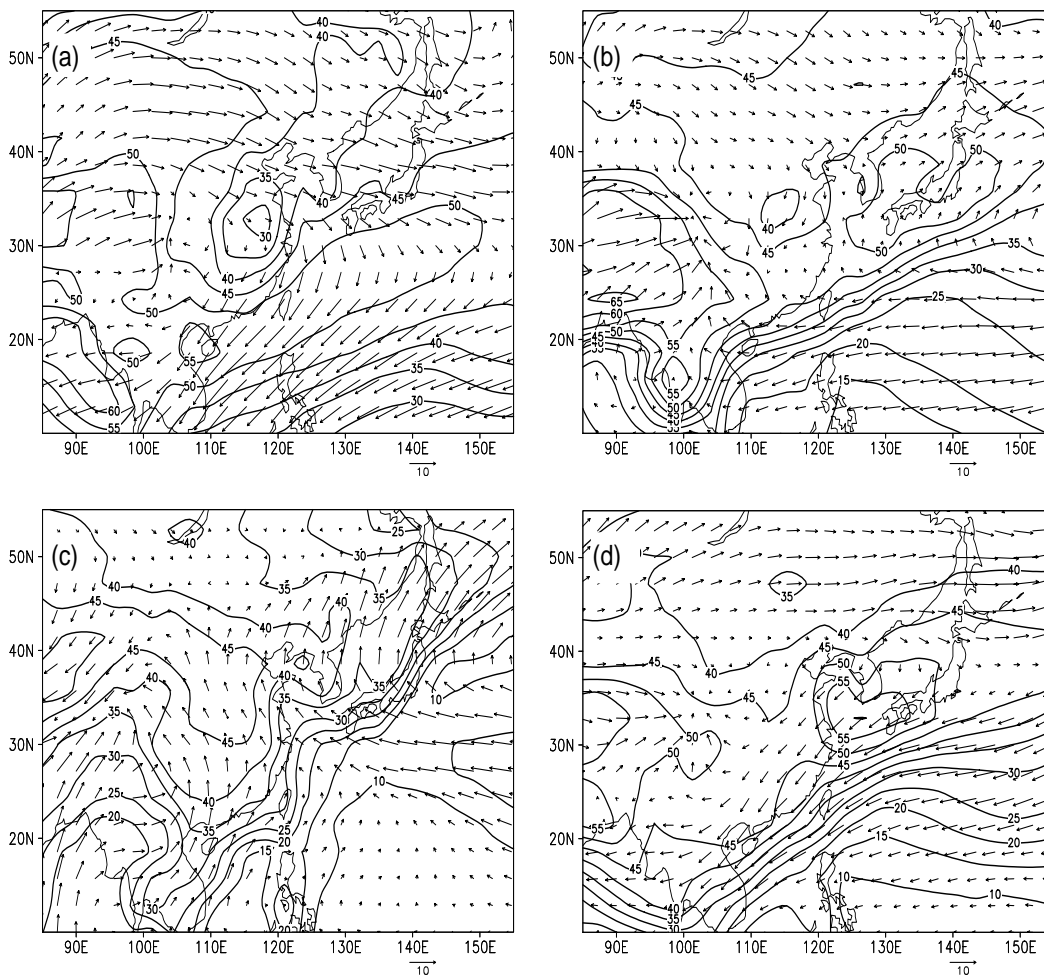
Fig. 2. Monthly average horizontal distributions of O_3 mixing ratios (ppbv) and monthly wind fields (units: m s^{-1} ) at a height of about 30 m above ground in (a) January (b) April (c) July (d) October.
