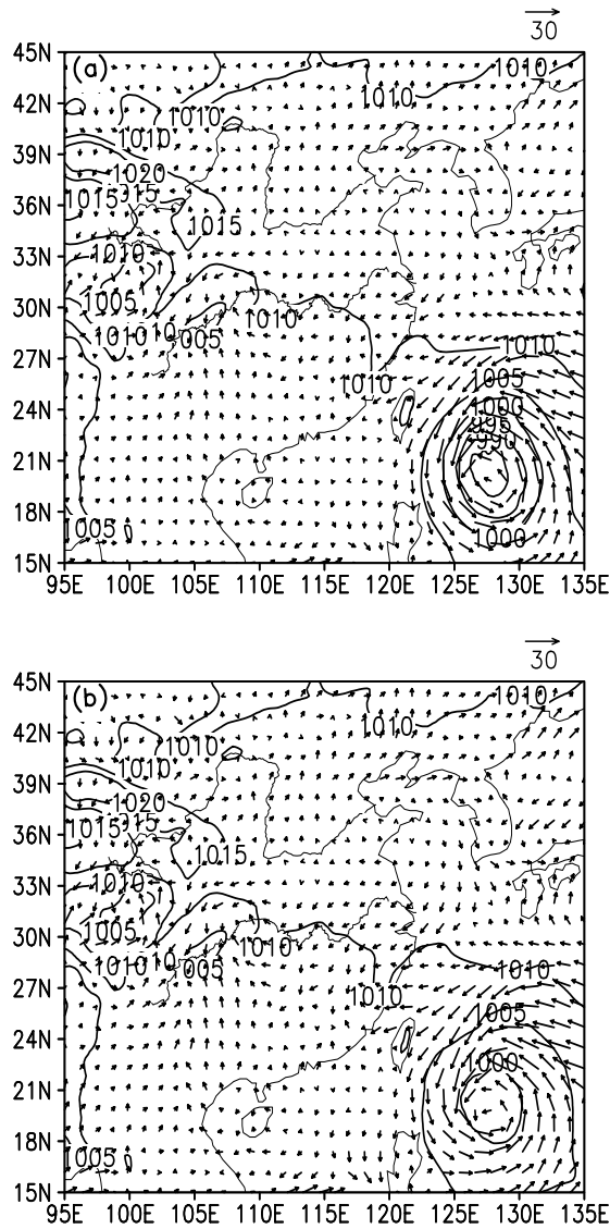
Fig. 1. 10-m wind field ( \text{m s}^{-1} ) and sea-level pressure at 1200 UTC on 31 August 2003 for Typhoon Dujuan (a) with data assimilation and (b) without data assimilation. Contour interval: 5 hPa.
