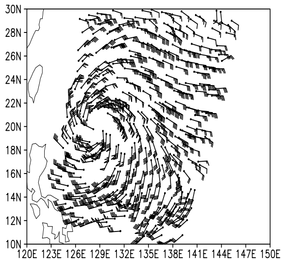
Fig. 3. Observed QuikSCAT 10-m wind vectors from 1030 UTC to 1330 UTC on 31 August 2003 for Typhoon Dujan. Each flag indicates 20 \text{ m s}^{-1} .
