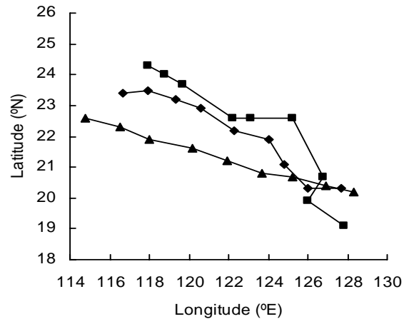
Fig. 11. Track forecasts of Typhoon Dujuan (0–48 h). (Output for each 6 h, the initial position of the real-time typhoon is located at 20.2°N, 128.3°E, \blacklozenge : with data assimilation, \blacksquare : without data assimilation and \blacktriangle : best-track)
