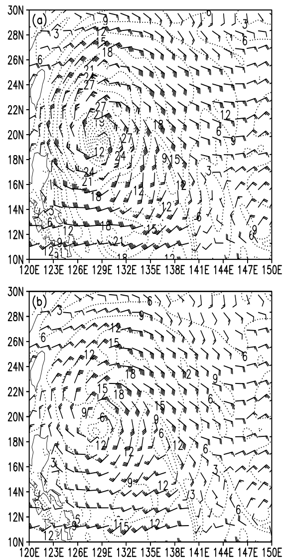
Fig. 2. Model-simulated 10-m wind vectors and isotach (dashed lines) at 1200 UTC on 31 August 2003 for Typhoon Dujuan (a) with data assimilation and (b) without data assimilation. Each flag indicates 20 \text{ m s}^{-1} , contour interval: 3 \text{ m s}^{-1} .
