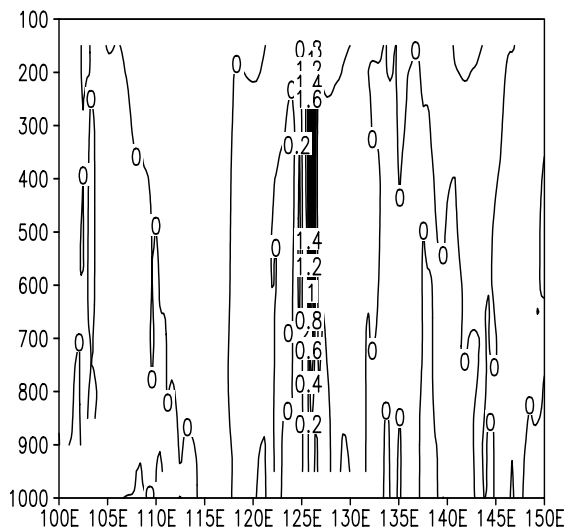
Fig. 5. As in Fig. 4, except for vertical wind speed. Contour interval: 0.2 \text{ m s}^{-1} .
