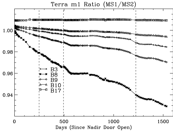
Fig. 5. Terra MODIS RSB response ( m_1 ) difference between two mirror sides for bands 3, 8, 9, 10, and 17.
