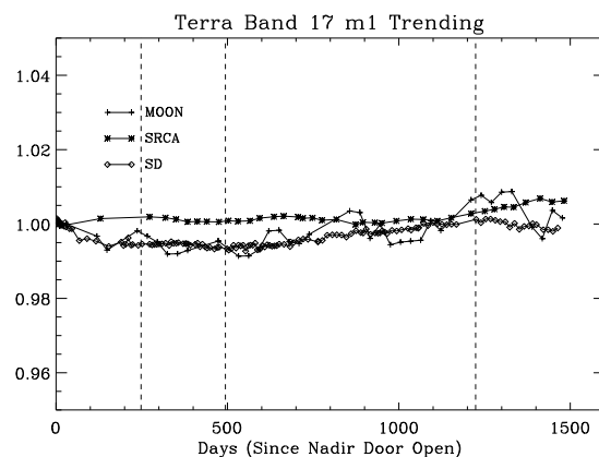
Fig. 4. Terra MODIS band 17 response trending at three different angles of incidence: SD, SRCA, and the Moon (through space view port)
