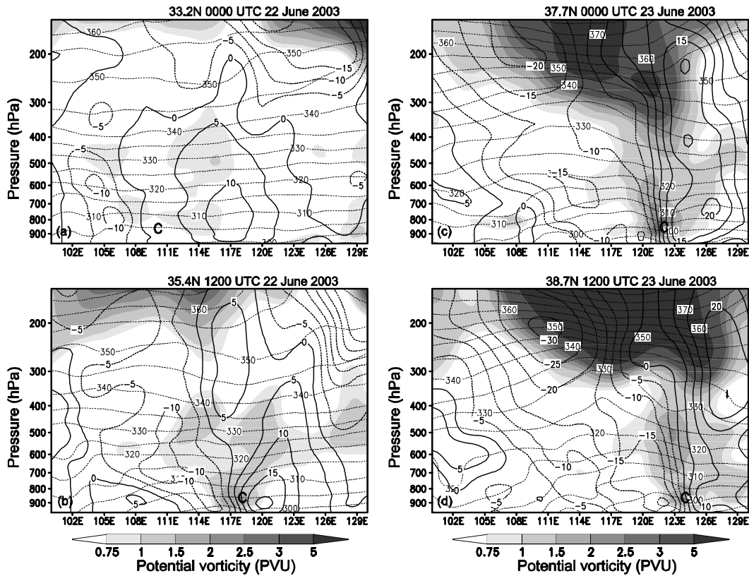
Fig. 5. Longitude-height cross sections of meridional wind (thick line, \text{m s}^{-1} ), PV (shaded, PVU), and potential temperature (thin dashed, K) along the cyclone center at 850 hPa for (a) 0000 UTC 22 June 2003; (b) 1200 UTC 22 June 2003; (c) 0000 UTC 23 June 2003; (d) 1200 UTC 23 June 2003. C is the location of the 850 hPa cyclone center.
