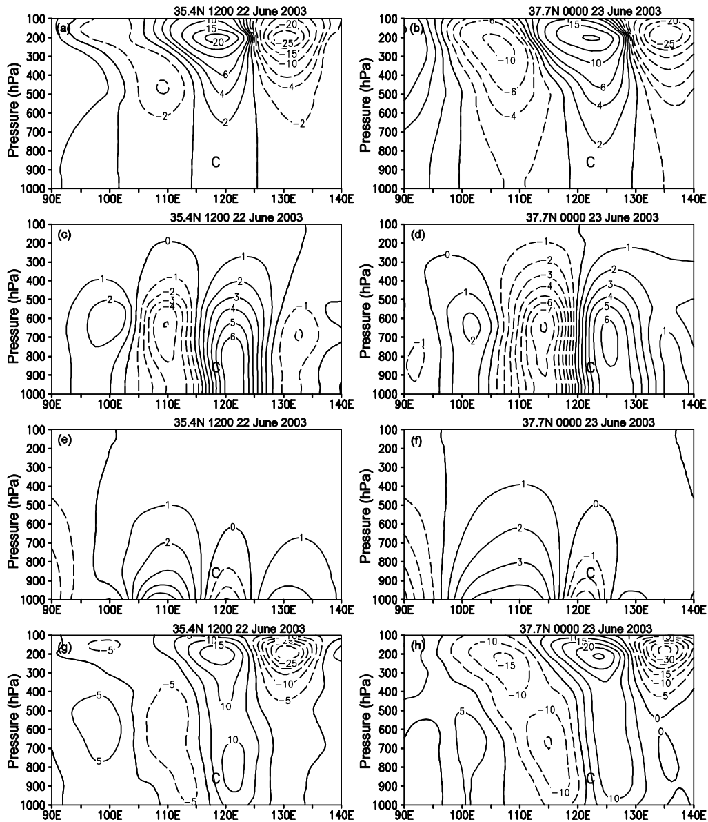
Fig. 7. As in Fig. 6 except for meridional wind (unit: \text{m s}^{-1} ).
