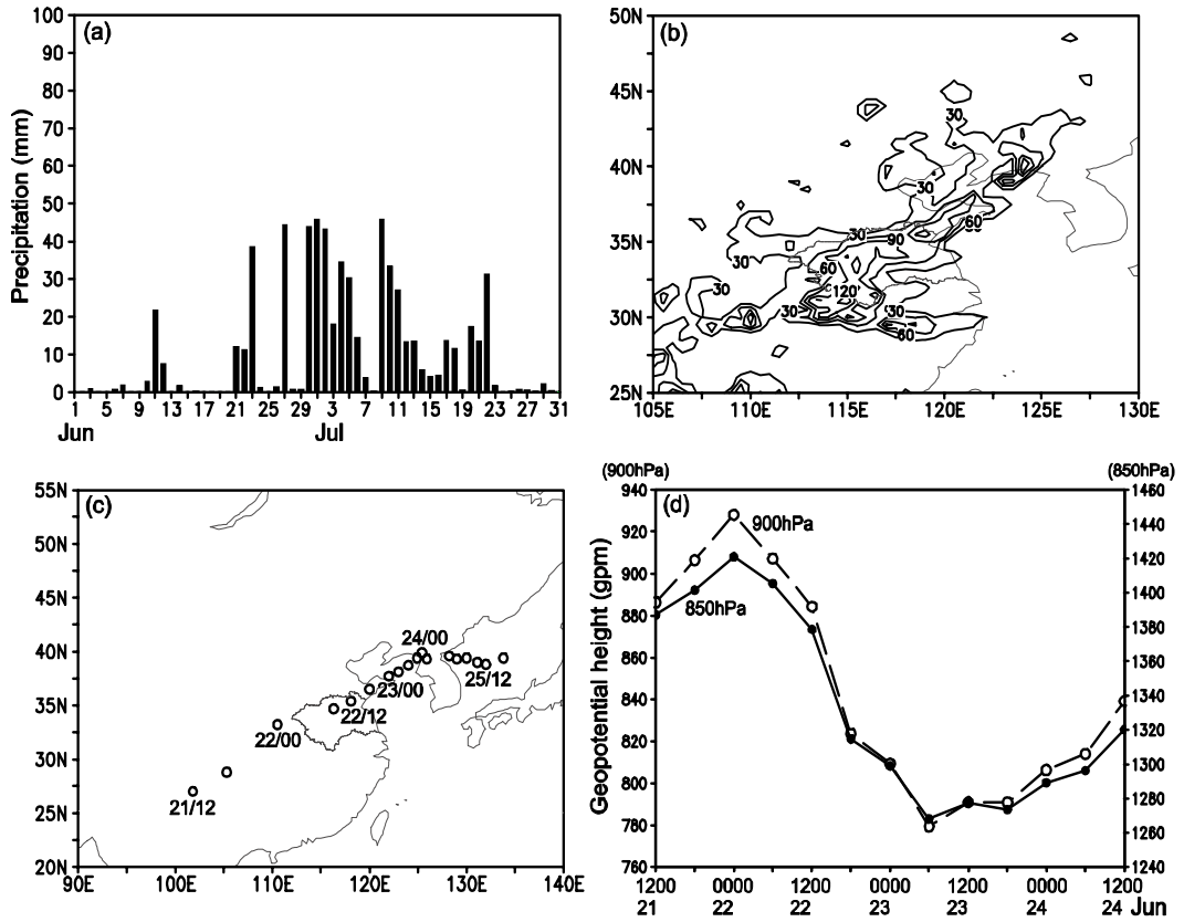
Fig. 1. (a) The evolution of averaged daily precipitation of the Huaihe River valley ( 31.5^{\circ} – 34.5^{\circ} N, 115^{\circ} – 120^{\circ} E) during June and July 2003. (b) Distribution of accumulative precipitation from 0000 UTC 21 to 0000 UTC 24 June 2003 with a contour interval of 30 mm. (c) The path of the cyclone at 850 hPa, where circles mark the locations of the cyclone center. (d) Intensity evolution of the 850 and 900 hPa geopotential heights at the cyclone center; y -coordinate is for the geopotential height (gpm).
