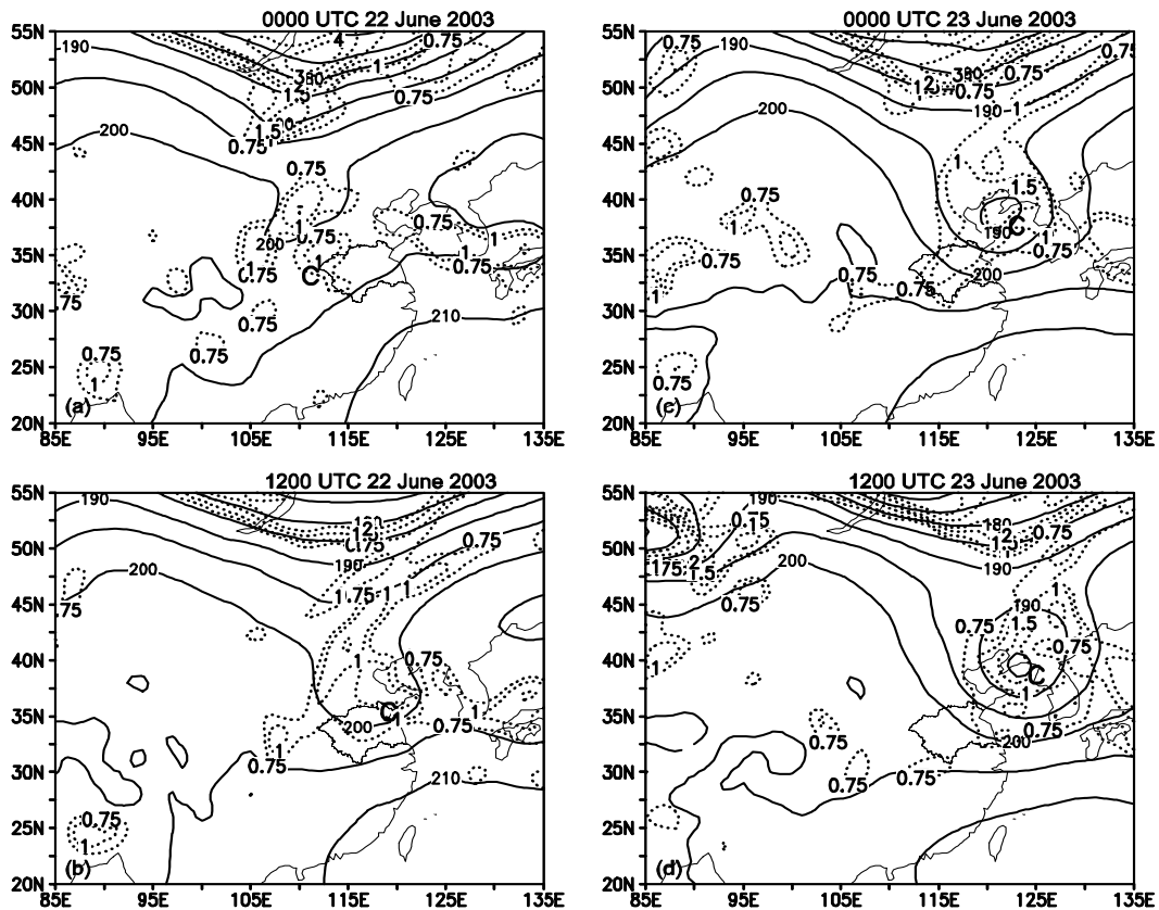
Fig. 4. Isentropic analyses at 320 K of the Montgomery streamfunction (solid, 200=3.200 \times 10^5 \text{ m}^2 \text{ s}^{-2} ) and PV (dotted, PVU) at (a) 0000 UTC 22 June 2003; (b) 1200 UTC 22 June 2003; (c) 0000 UTC 23 June 2003; (d) 1200 UTC 23 June 2003. C is the location of the 850 hPa cyclone center.
