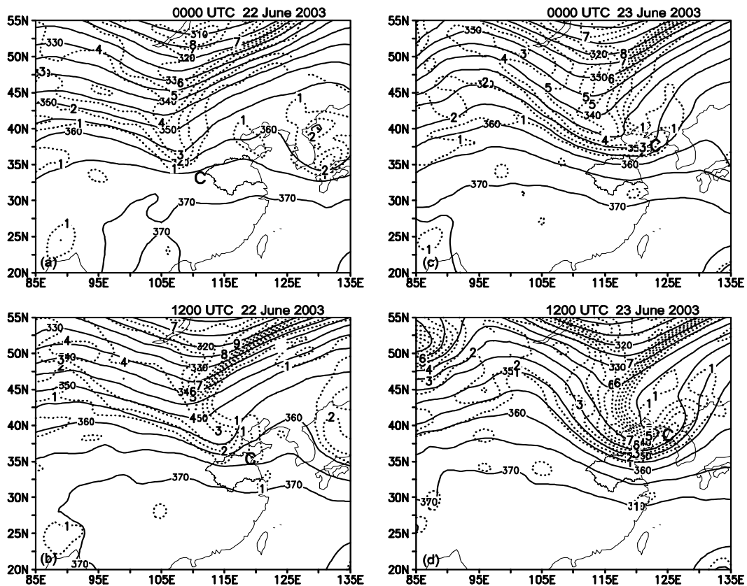
Fig. 3. Isentropic analyses at 340 K of the Montgomery streamfunction (solid, 340=3.340 \times 10^5 \text{ m}^2 \text{ s}^{-2} ) and PV (dotted, PVU) at (a) 0000 UTC 22 June 2003; (b) 1200 UTC 22 June 2003; (c) 0000 UTC 23 June 2003; (d) 1200 UTC 23 June 2003. C is the location of the 850 hPa cyclone center.
