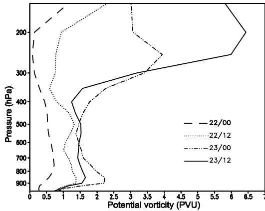
Fig. 2. Vertical distribution of the nine-point-averaged PV (PVU) of the cyclone center at 850 hPa.
