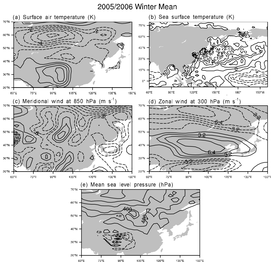
Fig. 2. 2005/06 winter (from December to February) mean anomalies of (a) temperature at 1000 hPa, (b) sea surface temperature, (c) meridional wind at 850 hPa, (d) zonal wind at 300 hPa, and (e) mean sea level pressure.
