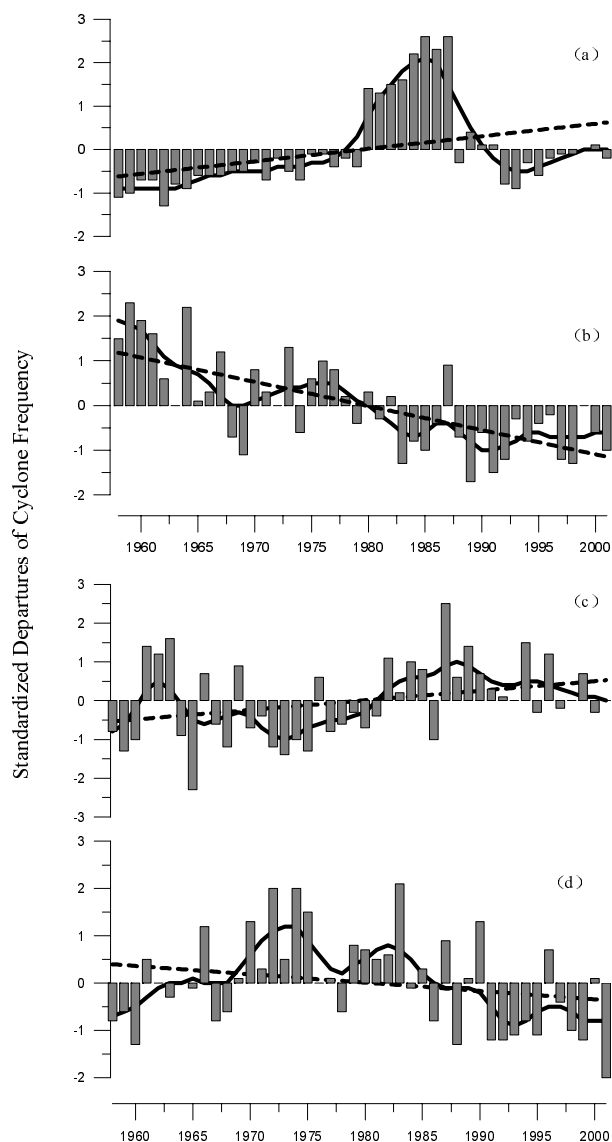
Fig. 6. Standardized departures (bars, relative to the average of 1958–2001), low frequency filtered signal (solid curves), and linear trend (dashed lines) of extratropical cyclone frequency for different regions in northern East Asia. Anomalies are calculated relative to 1958–2001 averages. Linear trends are not absolute frequency counts per decade. (a) 45^{\circ} – 50^{\circ} N, 90^{\circ} – 110^{\circ} E, trend: 0.29 (10\text{yr})^{-1} ; (b) 40^{\circ} – 45^{\circ} N, 90^{\circ} – 110^{\circ} E, trend: -0.54 (10\text{yr})^{-1} ; (c) 50^{\circ} – 55^{\circ} N, 110^{\circ} – 120^{\circ} E, trend: 0.25 (10\text{yr})^{-1} ; (d) 45^{\circ} – 50^{\circ} N, 110^{\circ} – 120^{\circ} E, trend: -0.18 (10\text{yr})^{-1} .
