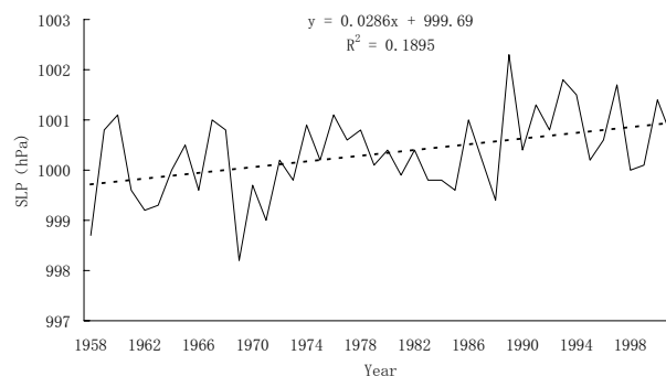
Fig. 7. Variations in intensities of northern East Asia extratropical cyclones as reflected by the averaged lowest center pressure for the entire lifetime of each cyclone.
