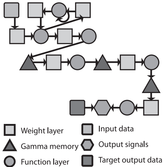
Fig. 2. Configuration of the neural network used in this study. The components used were assembled using Synapse (Peltarion).
