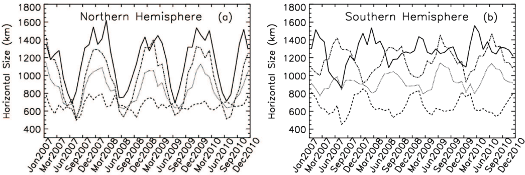
Fig. 7. Monthly time series of mean WDCS over the four-year period for different zonal bands in (a) the NH and (b) the SH. The dotted line represents WDCS over all zonal bands; the dashed line is for 0°–30°; the dash-dot line is for 30°–60°; and the solid line is for 60°–90°.
