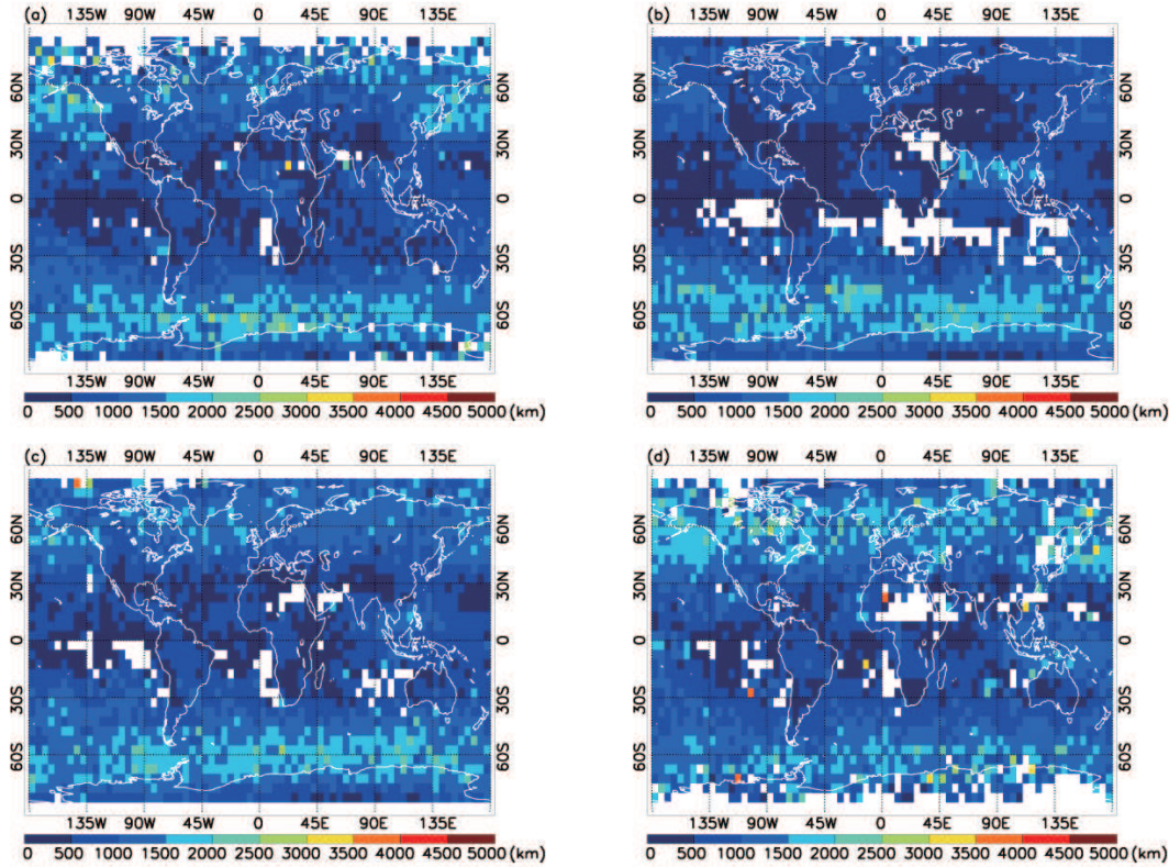
Fig. 8. Mean WDCS in each 5°×5° grid box over the four-year period for (a) NH spring/SH autumn, (b) NH summer/SH winter, (c) NH autumn/SH spring, and (d) NH winter/SH summer. White grid boxes signify that no DCS were identified in that box.
