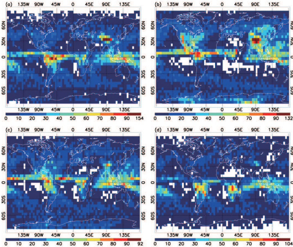
Fig. 3. Total number of DCS in each 5° × 5° grid box over the four-year period for (a) NH spring/SH autumn, (b) NH summer/SH winter, (c) NH autumn/SH spring, and (d) NH winter/SH summer. White grid boxes signify that no DCS were identified in that box.
