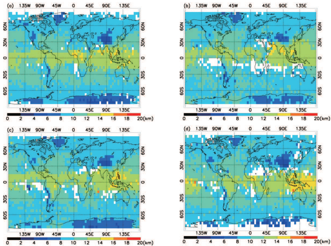
Fig. 6. Same as Fig. 5 but for mean DDCC.
