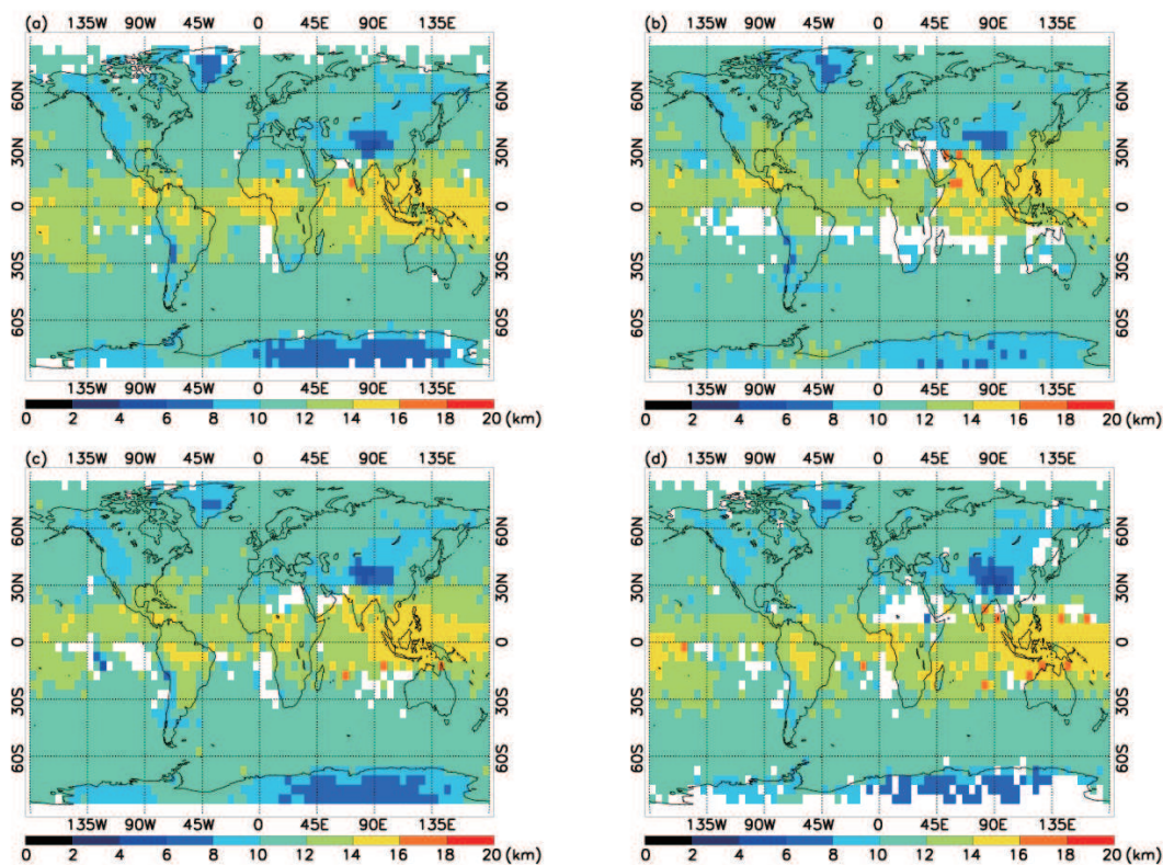
Fig. 5. Mean TDCC in each 5^{\circ} \times 5^{\circ} grid box over the four-year period for (a) NH spring/SH autumn, (b) NH summer/SH winter, (c) NH autumn/SH spring, and (d) NH winter/SH summer. White grid boxes signify that no DCS were identified in that box.
