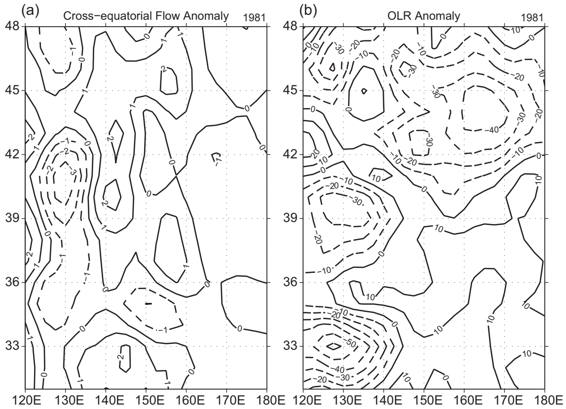
Fig. 9. Longitude–pentad cross section of the 850 hPa (a) cross-equatorial flow anomaly (units: \text{m s}^{-1} ) and (b) OLR anomaly along 15^\circ\text{N} (units: \text{W m}^{-2} ) during summer 1981. The numbers on the ordinate represent the Julian pentad.
