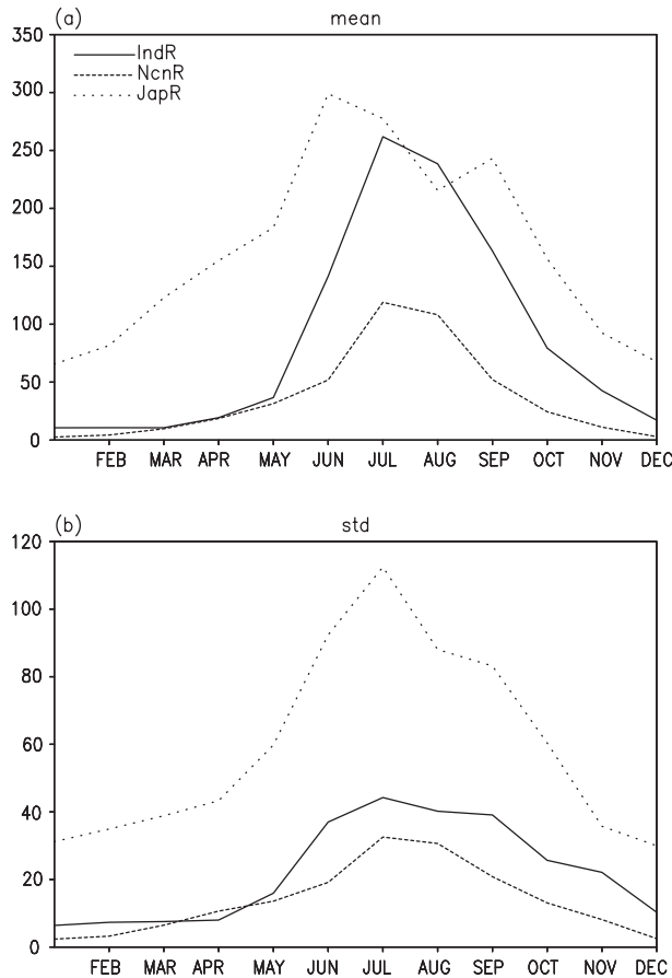
Fig. 1. (a) Climatological mean and (b) standard deviation of monthly area-mean Indian rainfall (IndR, solid curve), northern China rainfall (NcnR, dashed curve), and southern Japan rainfall (JapR, dotted curve) based on gridded CRU TS3.23 rainfall data for the period 1901–2014. The domains for obtaining area-mean rainfall are denoted by boxes in Fig. 2. Units: mm month -1 .
