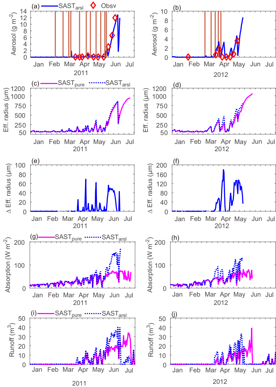
Fig. 8. Comparison between SAST pure (purple line) and SAST arsl (blue dashed line) in terms of (a, b) the aerosol mass distribution at the top snow layer (blue line) against observations (red diamonds), where brown bars are marked as the dates when aerosol loading occurs; (c, d) the effective radius at the top snow layer; (g, h) the radiative absorption at the top snow layer; and (i, j) runoff. Panels (e, f) show the difference in effective radius between SAST pure and SAST arsl at the top snow layer (blue line). Panels (a, c, e, g, i) are the results for 2011, while (b, d, f, h, j) are for 2012.
