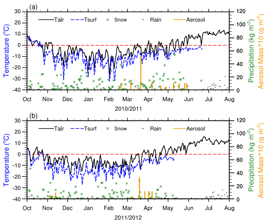
Fig. 2. Daily variations of air temperature (black line), surface temperature (blue dashed line), snow precipitation (green stars), rain precipitation (black dots), and aerosol loading mass (orange bars) at the SASP in 2010–12.
