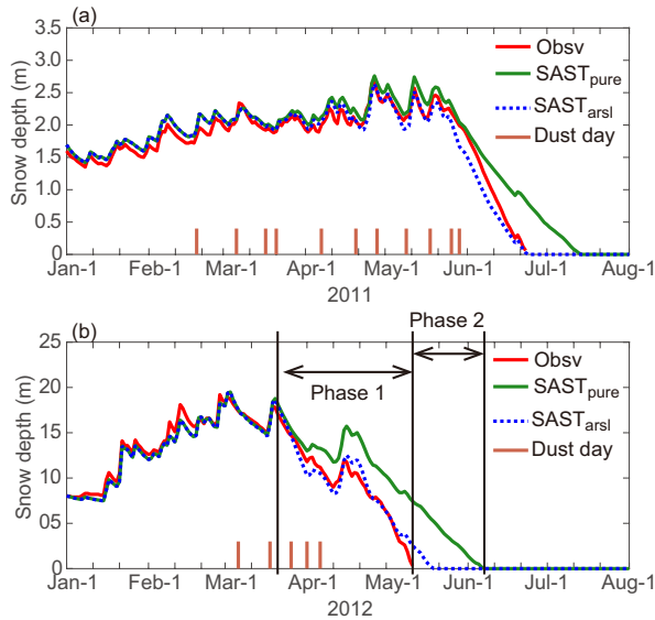
Fig. 7. Comparison of snow depth between simulations and observations (red line) at the SASP in 2011 and 2012. The blue dashed line is the simulation by SAST arsl , meaning snow containing aerosols. The green line is SAST pure , meaning clean snow. Brown bars are marked as the dates when aerosol loading occurs.
