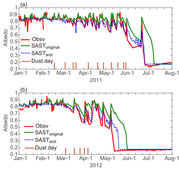
Fig. 4. Comparison of snow albedo between simulations by SAST_{original} (green line) and SAST_{arsl} (blue dashed line) against observations (red line) at the SASP in 2011 and 2012. Brown bars are marked as the dates when aerosol loading occurs.
