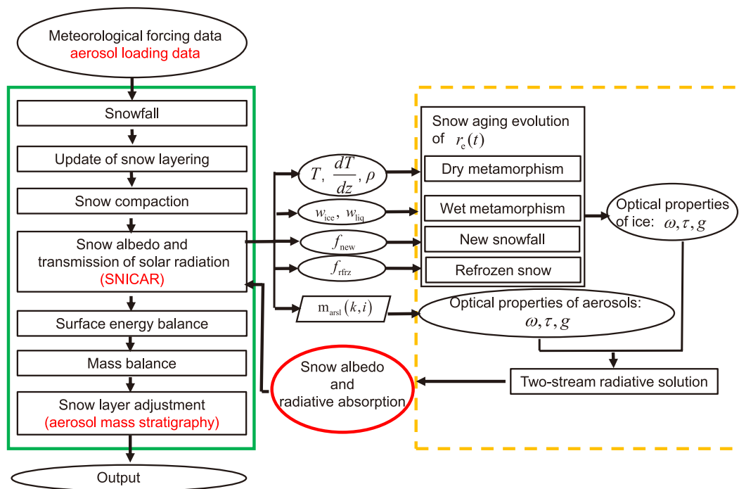
Fig. 1. Flow chart of the coupling of the SNICAR scheme into the SAST model. Inputs and outputs are presented in oval shapes. The green box indicates physical processes in the SAST model, while the orange dashed box relates to the SNICAR scheme.
