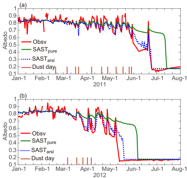
Fig. 6. Comparison of snow albedo between simulations and observations (red line) at the SASP in 2011 and 2012. The blue dashed line is SAST arsl , meaning snow containing aerosols. The green line is SAST pure , meaning clean snow. Brown bars are marked as the dates when aerosol loading occurs.
