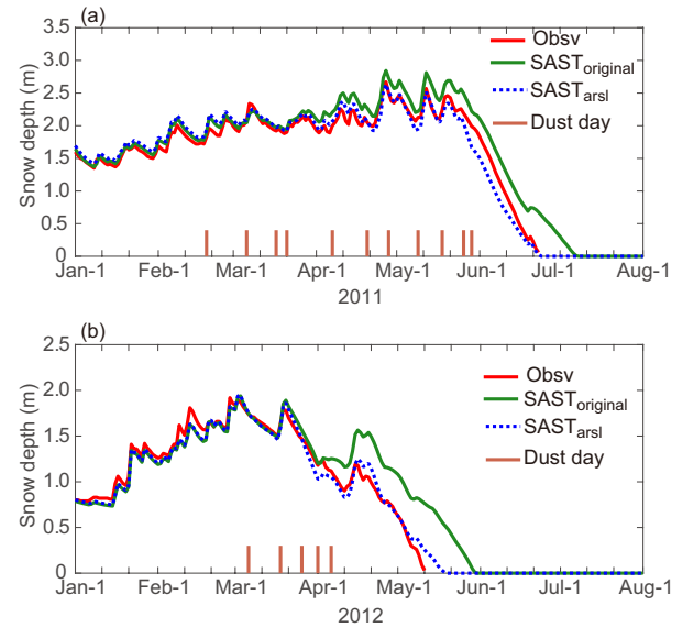
Fig. 5. Comparison of snow depth between simulations by SAST_{original} (green line) and SAST_{arsl} (blue dashed line) against observations (red line) at the SASP in 2011 and 2012. Brown bars are marked as the dates when aerosol loading occurs.
