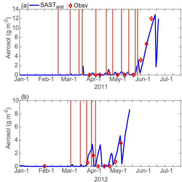
Fig. 3. Comparison of aerosol mass between simulations by SAST arsl (blue line) in the top snow layer and observations in the top 3 cm (red diamonds). Brown reference lines are marked as the dates when aerosol loading occurs. The simulations are the results of the daily mean of the model outputs (hourly).
