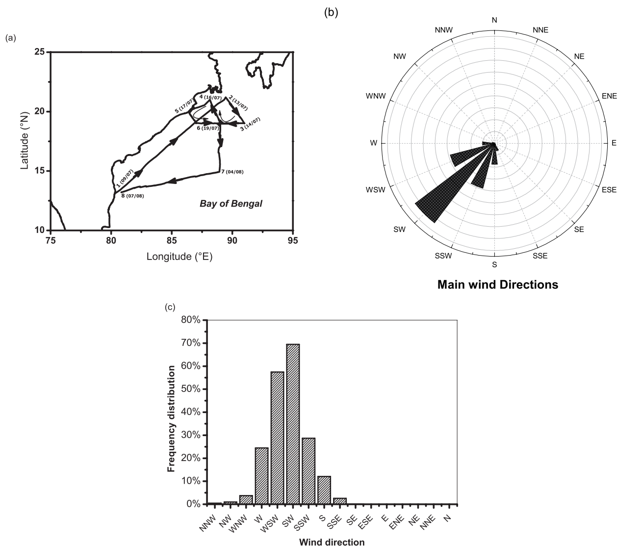
Fig. 1. (a) SK-296 track positions. (b) Wind-rose diagram (black shadings mark the southwest and south-southwest winds). (c) Frequency distribution of winds.
