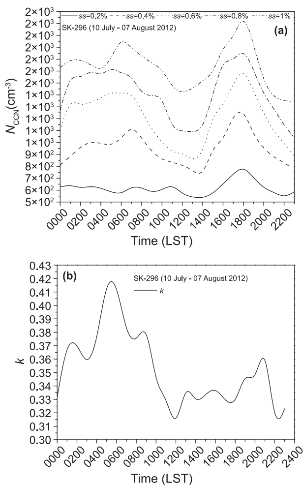
Fig. 2. Diurnal patterns of (a) the CCN distributions at each supersaturation level from 0.2% to 1% (in steps of 0.2%) and (b) k , for the measurement period from 10 July to 7 August 2012.
