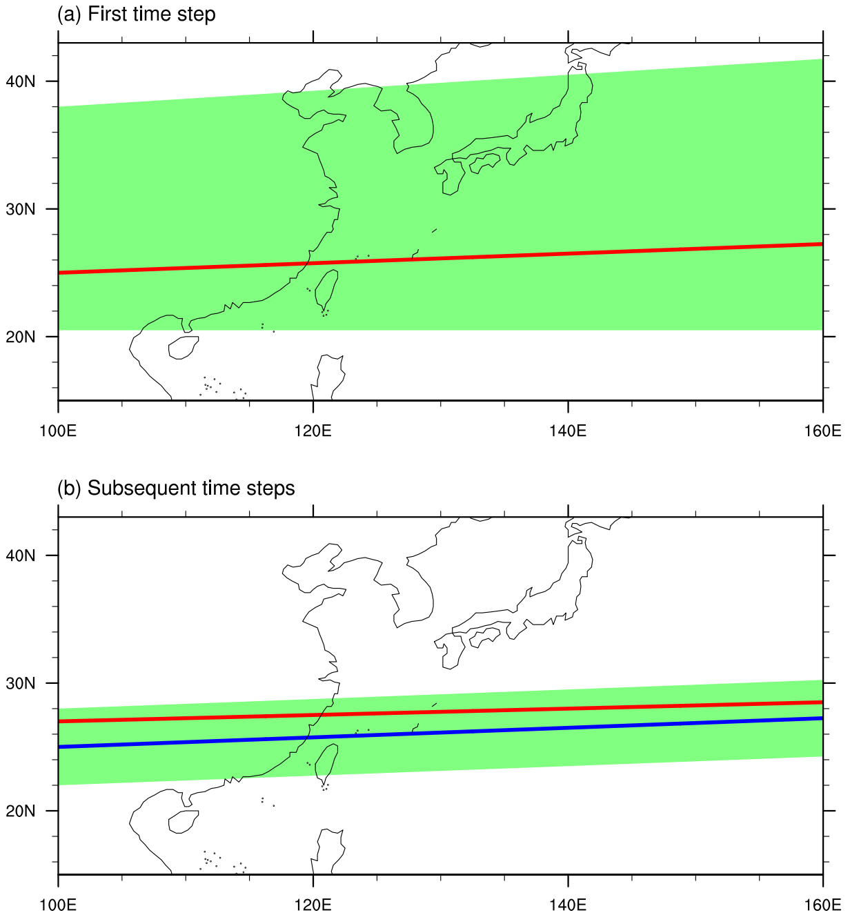
Fig. S1. Schematic diagram of MYF detection (a) for the first time step and (b) for the subsequent time steps (see section 3.2 and Fig. 1 for more information). Green regions indicate the search regions. Red lines indicate the MYF detected at the current time step. Blue line indicates the MYF detected at the previous time step.
